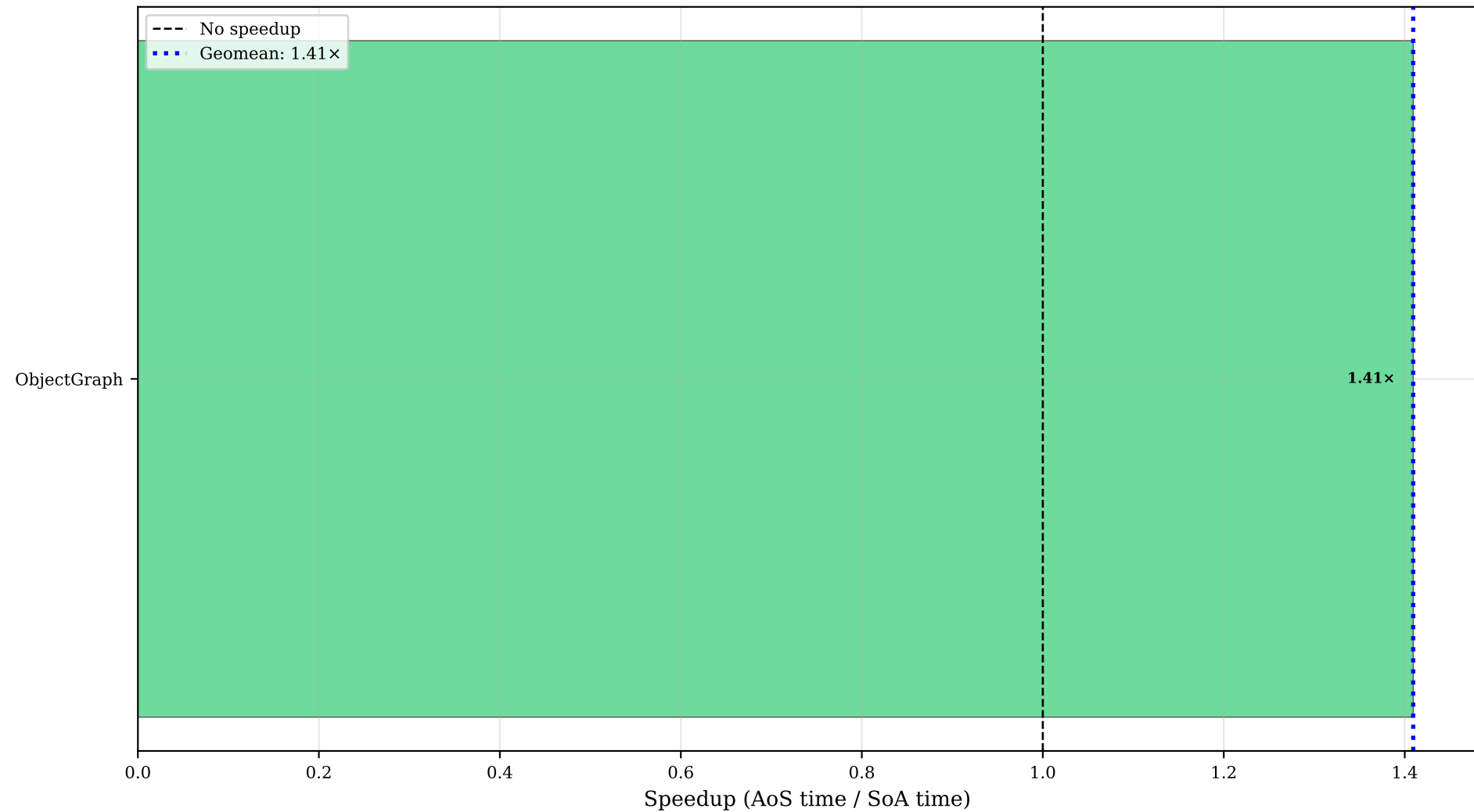
sumObjIds (fold): Speedup Across All Programs (>1.0 means SoA is faster)
