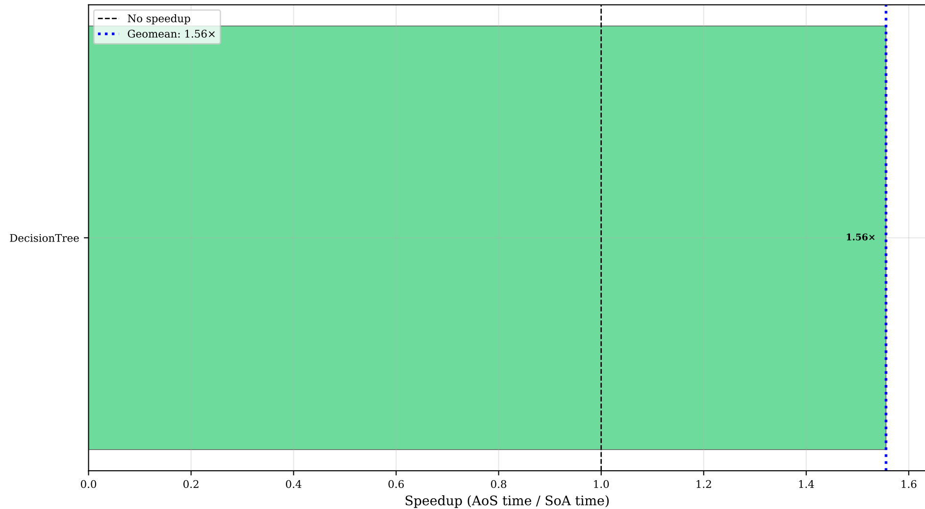
sumSamples (fold): Speedup Across All Programs (>1.0 means SoA is faster)
