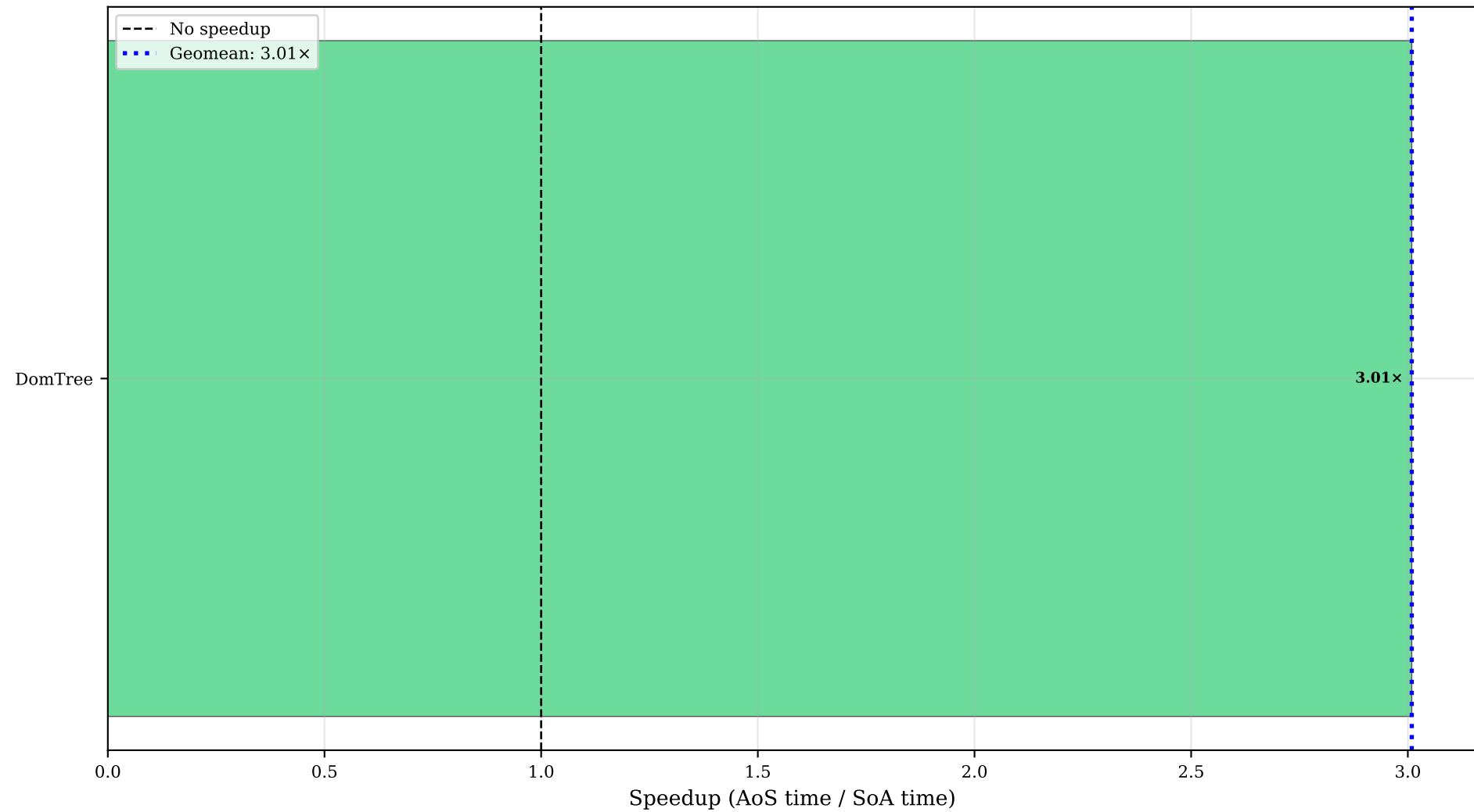
sumTextWidth (fold): Speedup Across All Programs ( >1.0 means SoA is faster)
