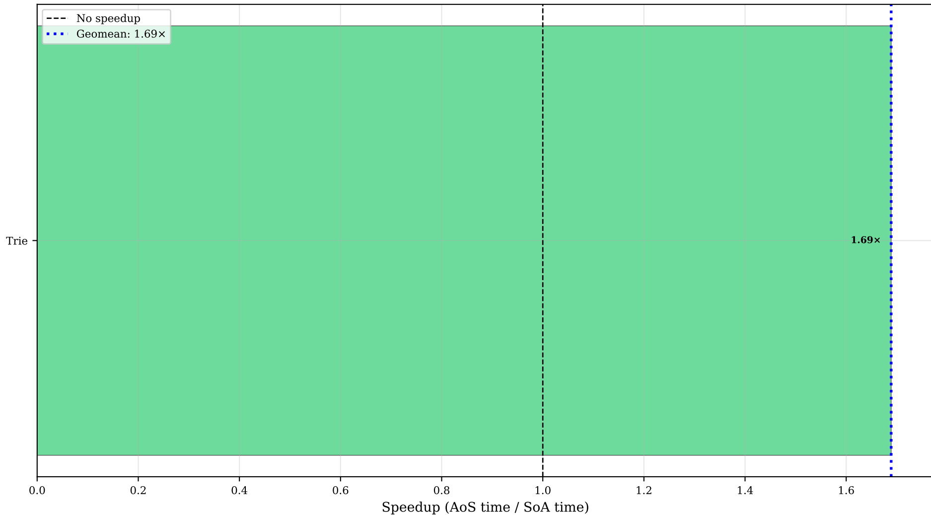
sum frequency (fold): Speedup Across All Programs (>1.0 means SoA is faster)
