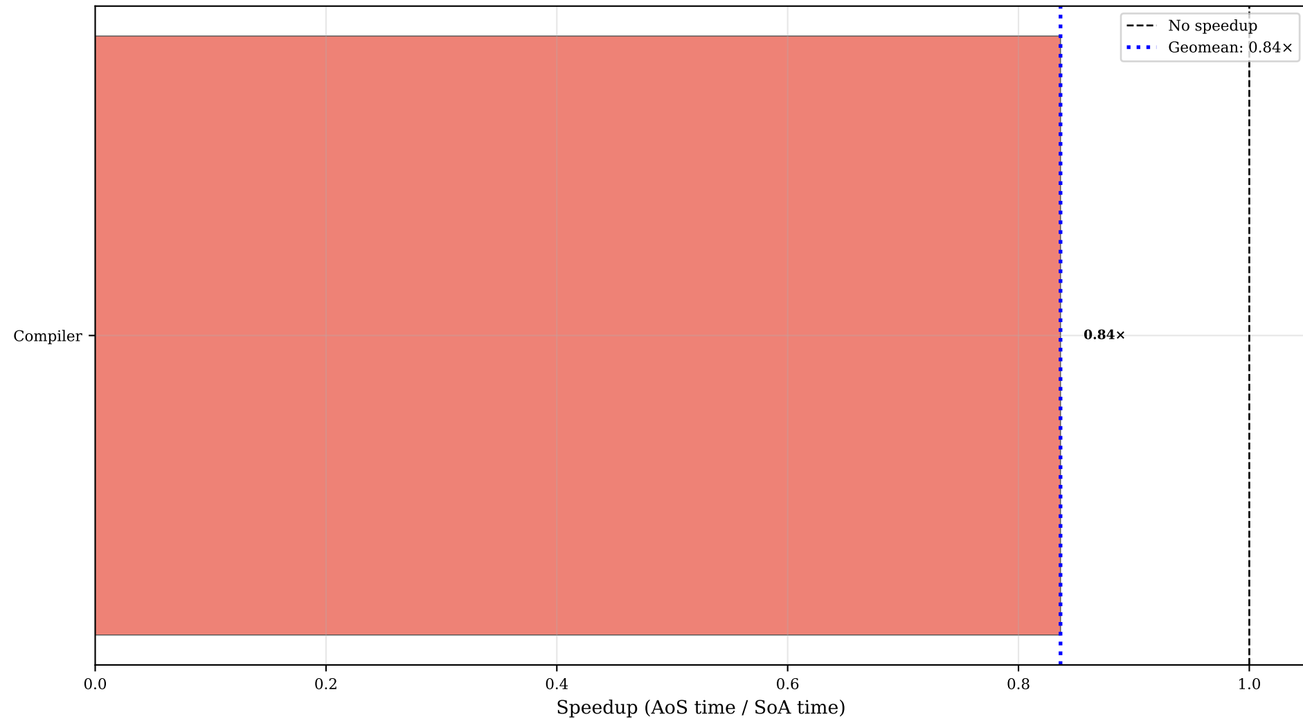
targetReturn (map): Speedup Across All Programs ( >1.0 means SoA is faster)
