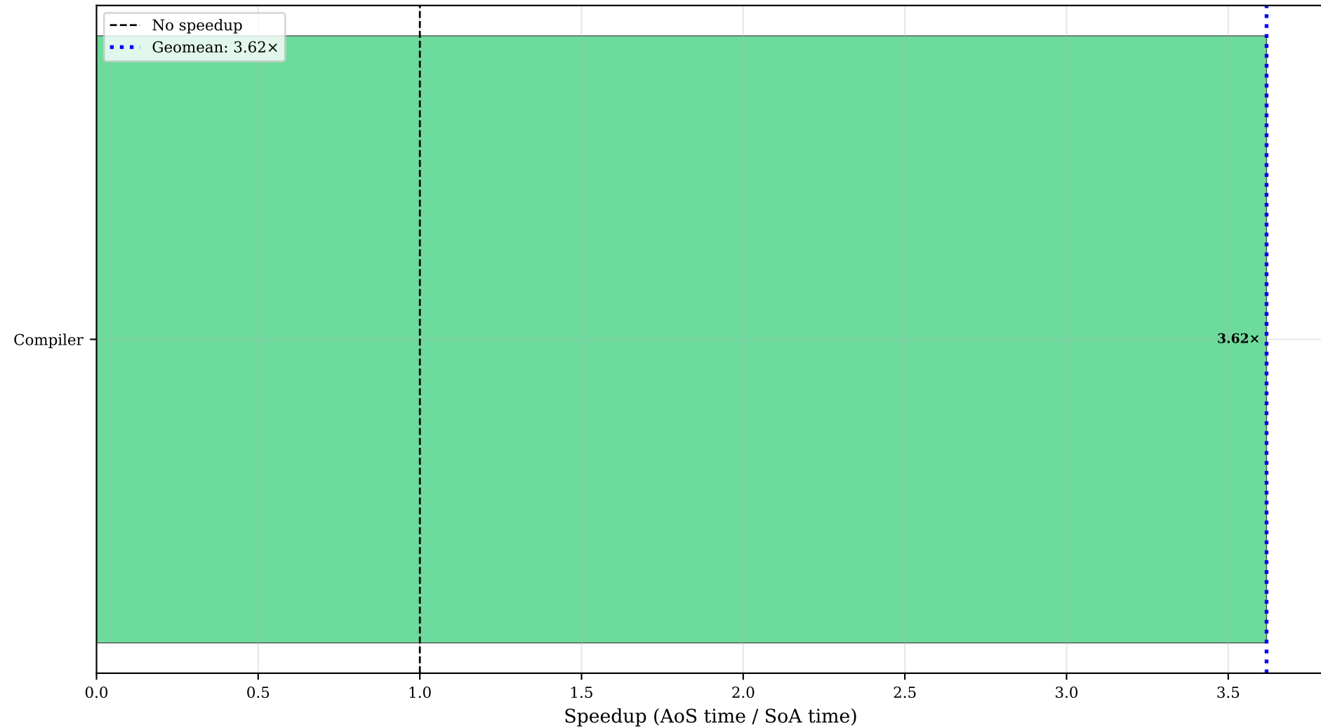
throughputModel (fold): Speedup Across All Programs (>1.0 means SoA is faster)
