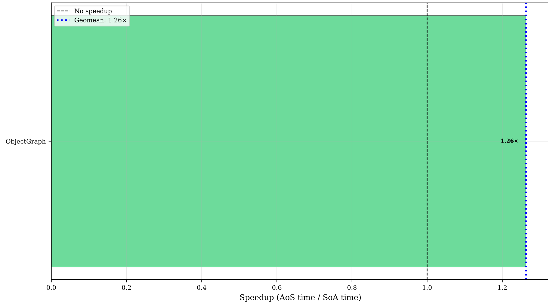
totalHeapSize (fold): Speedup Across All Programs (>1.0 means SoA is faster)
