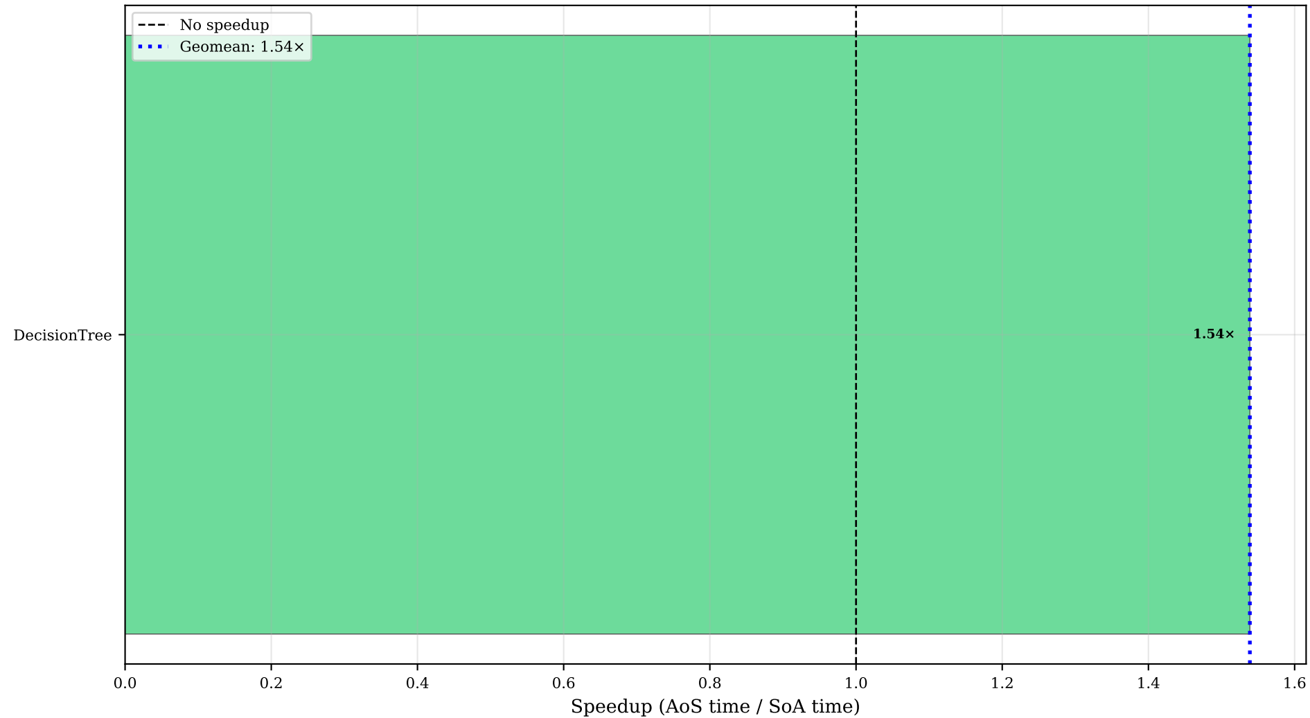
treeDepth (fold): Speedup Across All Programs (>1.0 means SoA is faster)
