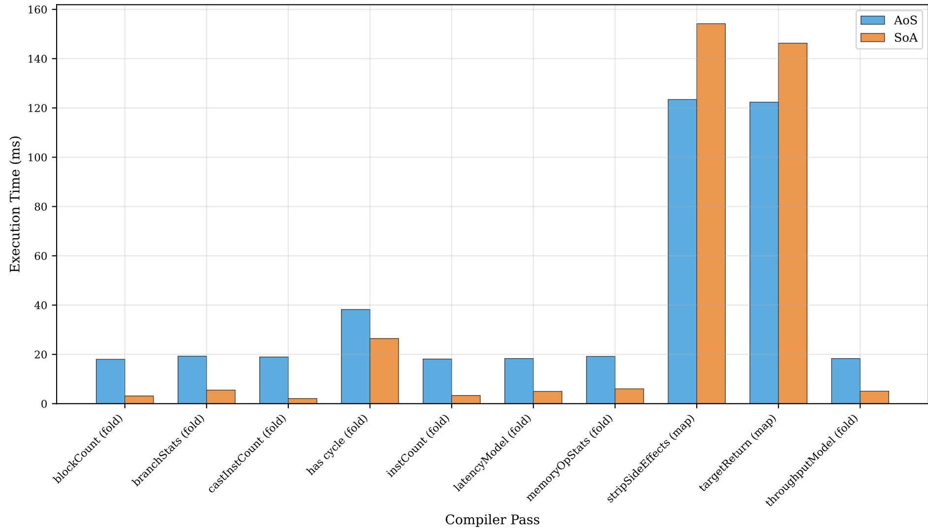
Compiler: All Passes Performance
