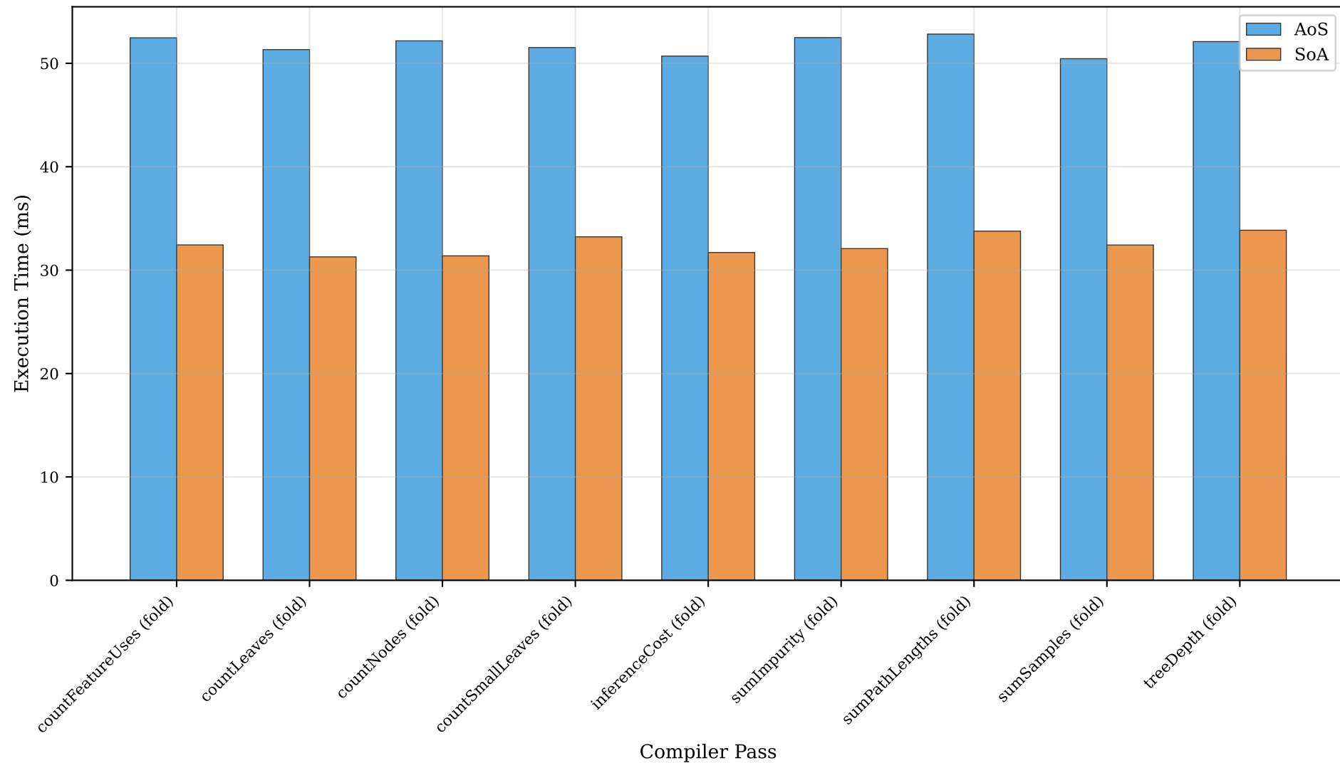
DecisionTree: All Passes Performance
