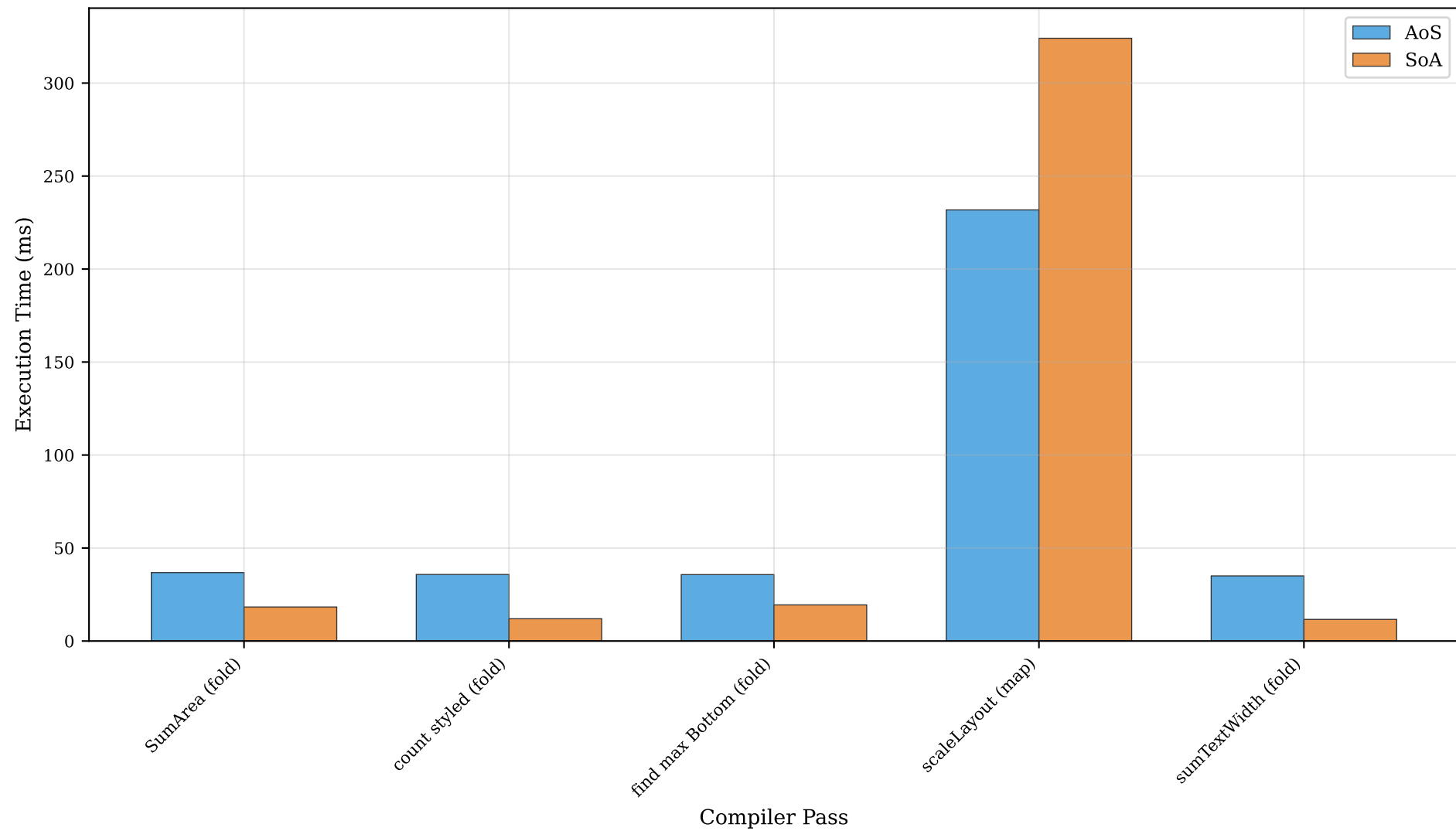
DomTree: All Passes Performance
