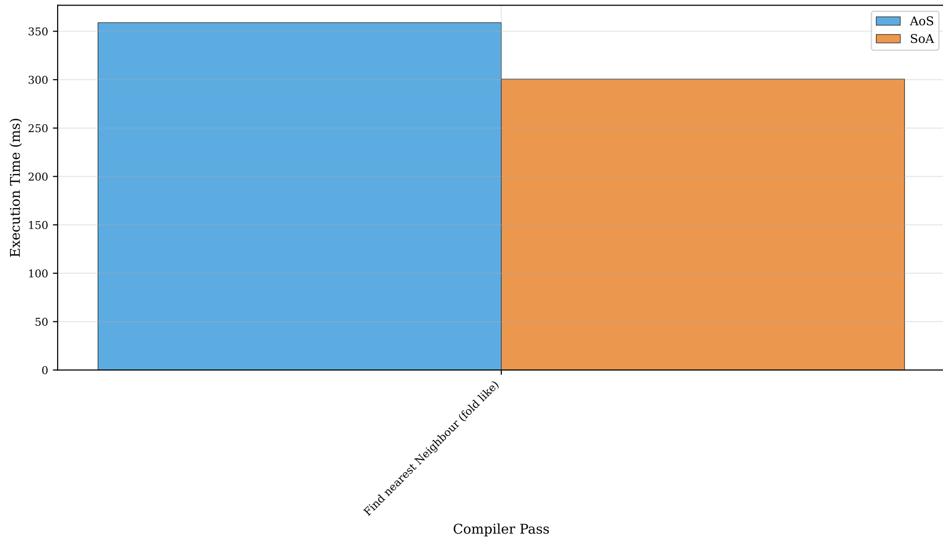
KDTree: All Passes Performance
