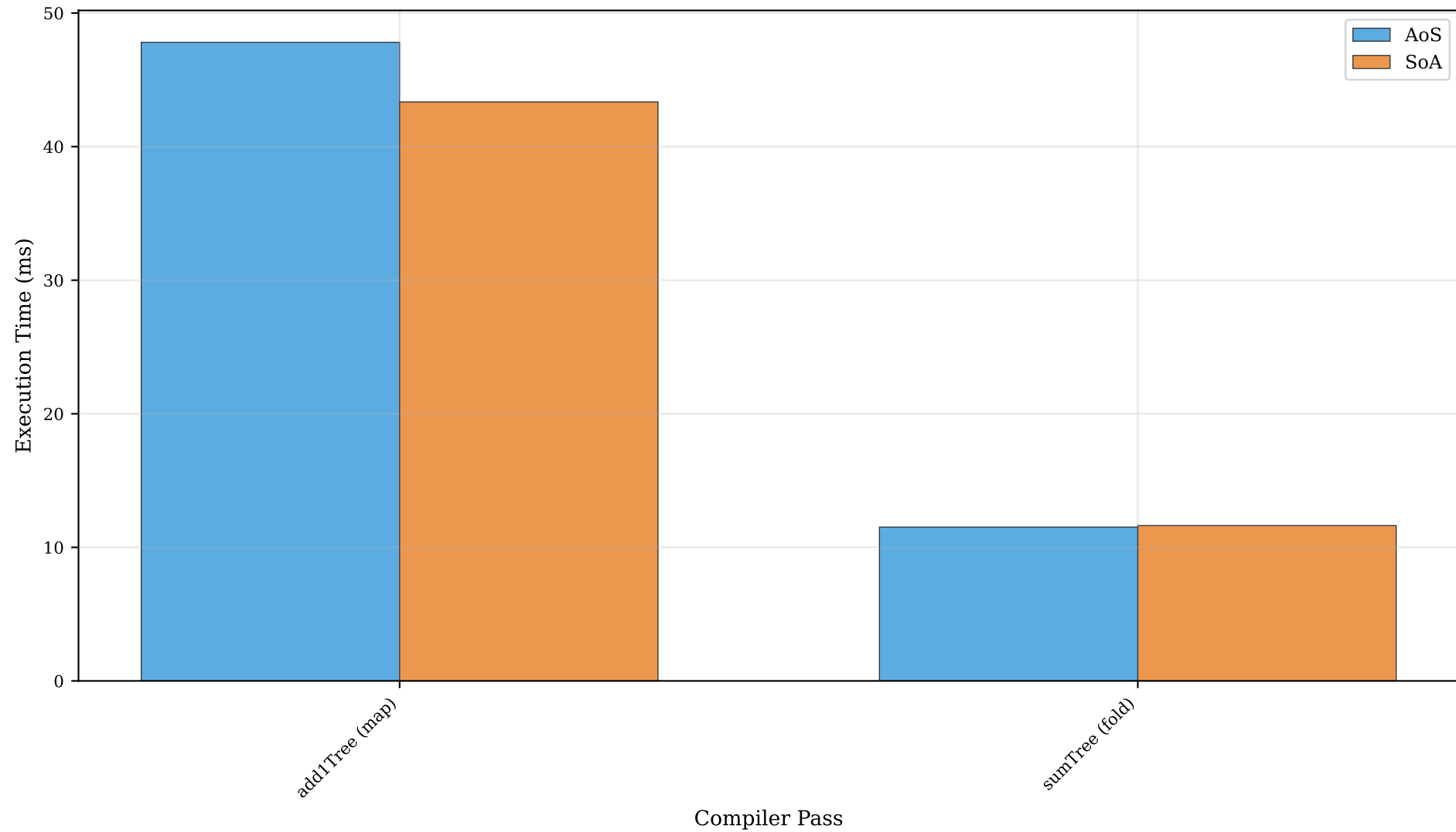
MonoTree: All Passes Performance
