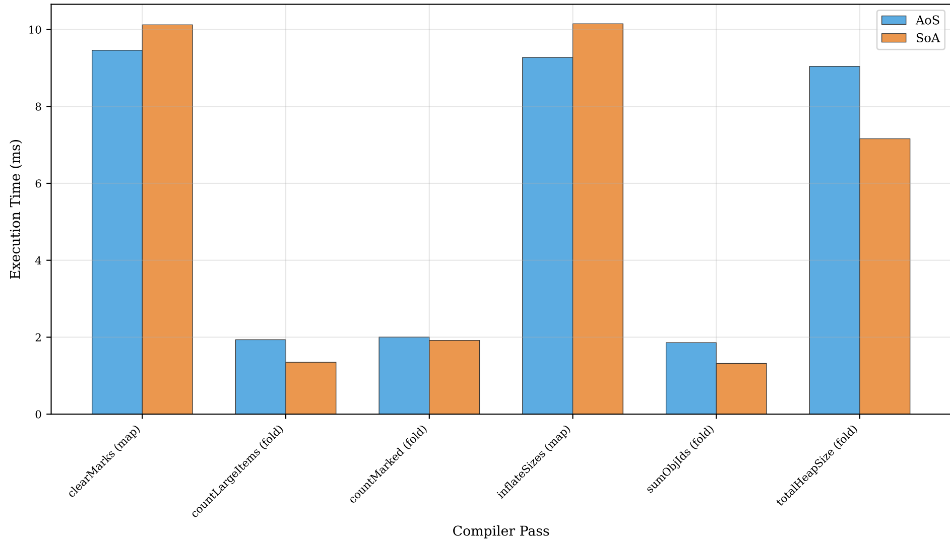
ObjectGraph: All Passes Performance
