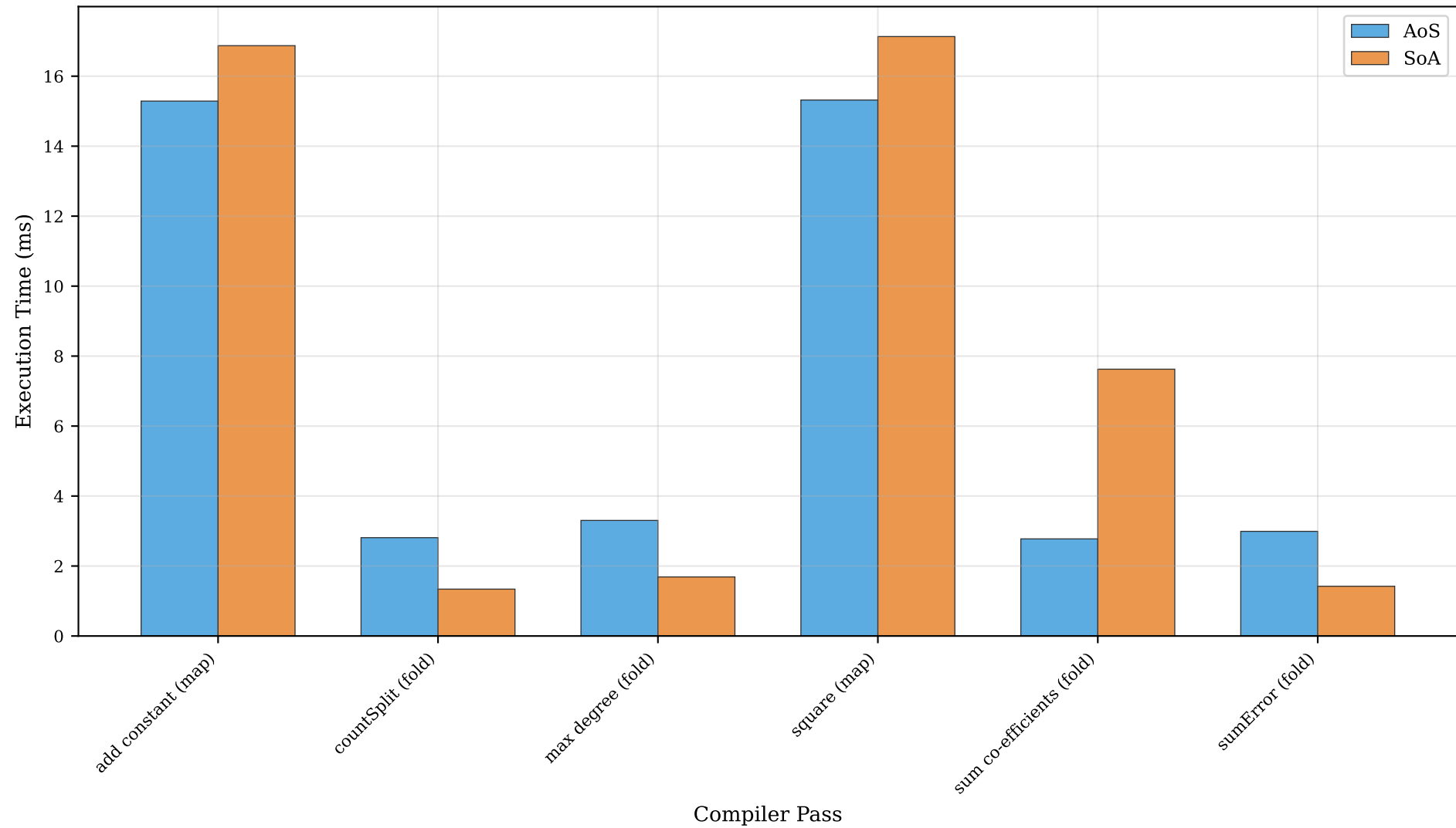
PiecewiseFunctions: All Passes Performance
