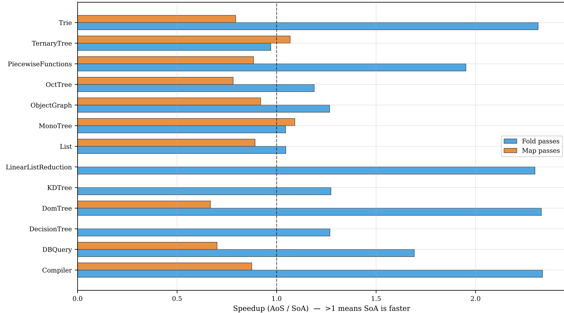
End-to-End Speedup: Fold vs Map Passes
