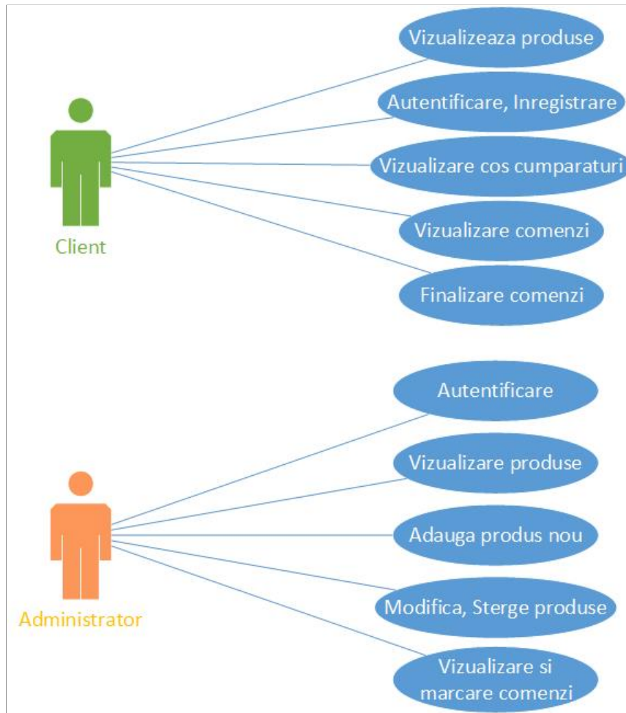
Figure 1: Use Case
