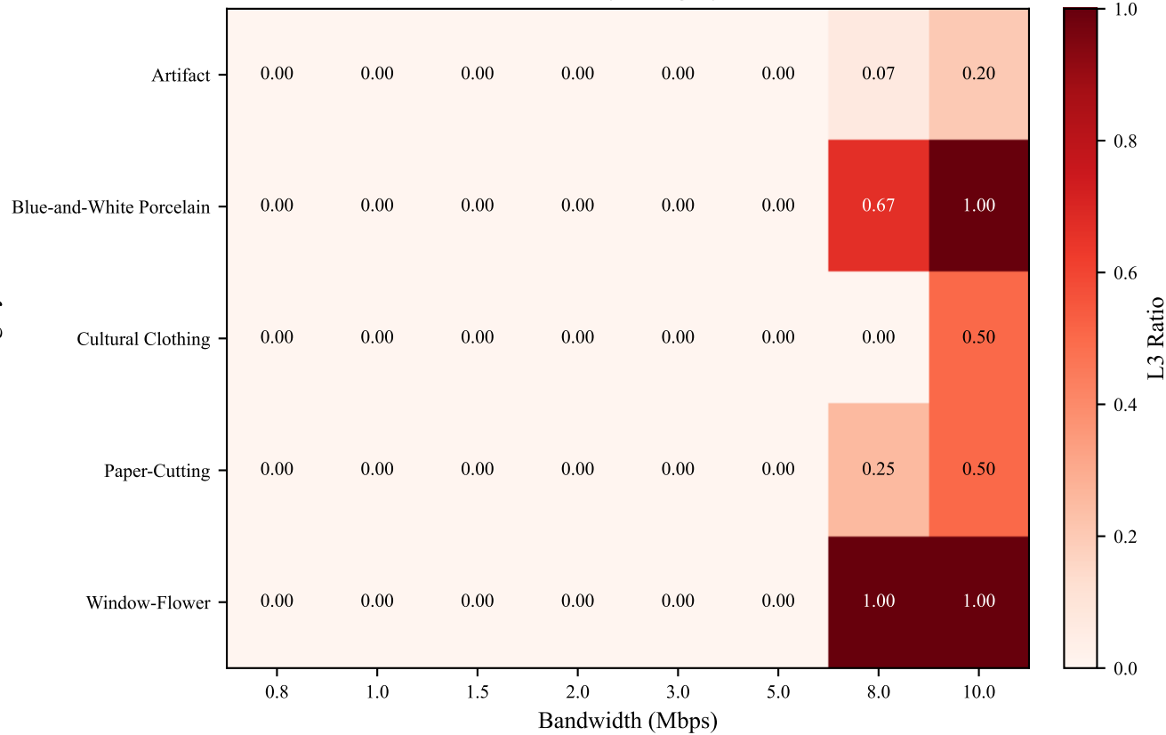
(c) L3 Selection Rate by Category and Bandwidth
