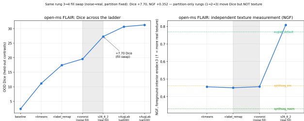
Figure 5. Downstream Dice (left) against an independent, segmentation-free measurement of texture fidelity (right, NGF gradient-orientation agreement with the source volume) across the rung sequence. The three noise-fill rungs sit flat at the texture floor while their Dice still rises – those gains come from richer contrast randomization, not texture. Both quantities jump together at the fill swap, which is the step the texture hypothesis predicts.
