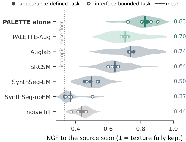
Figure 3. Texture kept by each augmentation: NGF similarity of the augmented volume to its source scan on the seven ablation tasks (violin: all scans, each averaged over 5 draws; dots: task means; bar: mean of the task means). The noise fill keeps only the partition edges; the real fill keeps the most.
