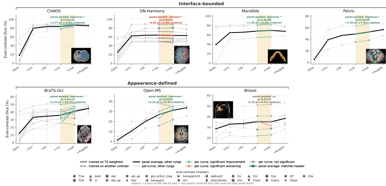
Figure 2. The one-variable test, one panel per task with a ladder, grouped by target type. Each thin line is one (training modality, held-out contrast) pair, external cohorts included; only its real-fill segment (shaded band) is colored, by that pair’s significance: teal improves, red worsens, grey is not significant. The bold black line is the panel average, colored by the panel test annotated above it: one paired Wilcoxon test on patients (each counted once across contrasts and models) pooling all training modalities, Holm-corrected across the seven panels. rel. = panel gain / mean noise-fill Dice. Two of the three appearance-defined panels improve significantly and strongly (BraTS-GLI +14.7%, p = 3.6 \times 10^{-11} ; Open-MS +15.8%, p = 0.023 ) and Breast does not move. The interface-bounded panels move much less in relative terms: Pelvis (+7.3%), CHAOS (+3.9%) and Mandible (+2.0%) gain, and ON-Harmony worsens (−1.0%; significant with its eight sessions as units, which come from four subjects). Solid/dashed = trained on a T1-weighted vs. other contrast; marker = held-out contrast. Per-row numbers in Tab. 4; HD95 in Fig. 4 and Tab. 10.
