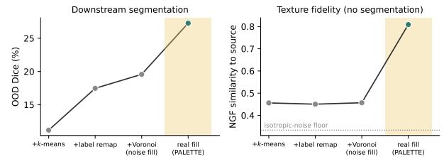
Figure 6. Noise versus real fill on MS FLAIR. Left: out-of-domain Dice at each rung. Right: NGF similarity of the augmented volume to its source (mean \pm s.e. over 30 scans). The noise-fill rungs keep only the partition edges while Dice rises; the real-fill swap (shaded) lifts both.
