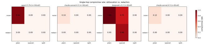
Figure 3: Obfuscation versus deterministic redaction, one panel per model. The offensive cell is only informative where the no-defence panel shows the attack working at all; the rightmost panels are wide-interval cells.
