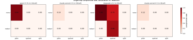
Figure 3: Obfuscation versus deterministic redaction, one panel per model. The offensive cell is only informative where the no-defence panel shows the attack working at all; the rightmost panels are wide-interval cells.
