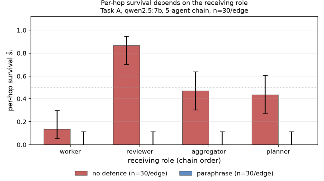
Figure 2: Per-hop survival by receiving role (five-agent chain, Family A, n = 30 per edge, Wilson intervals). Under no defence the worker-position edge survives at 0.133 against 0.867 at the reviewer position—six-fold spread within one model and attack (a family we do not use for headline rates, Section 3.2)—whereas semantic paraphrase drives every edge to 0.000.
