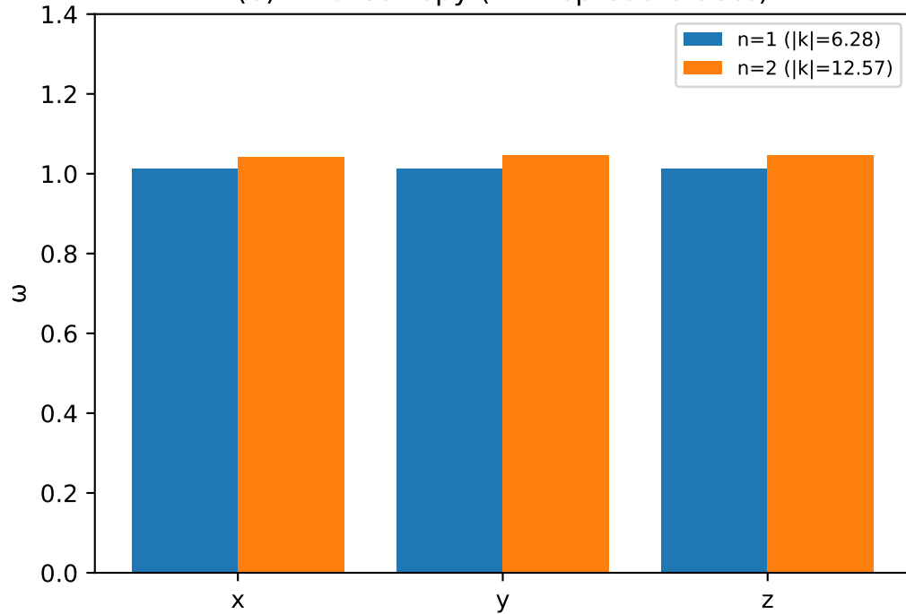
(b) Axis isotropy (n=2 spread 0.38%)
