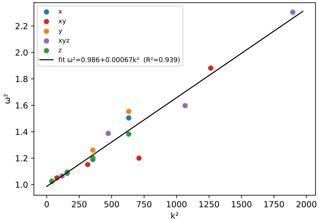
(a) 3D dispersion: \omega^2 = m^2 + c^2 k^2 ( m^2_{in}=1 )
