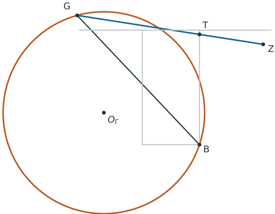
(a) The prepared circle solves the quadratic
