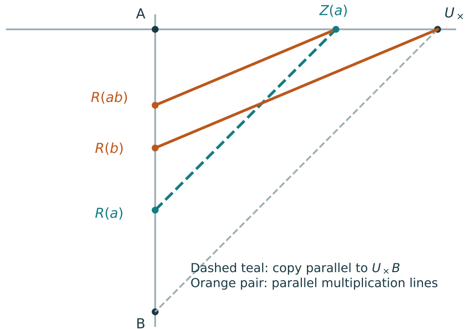
(a) One geometric multiplication
