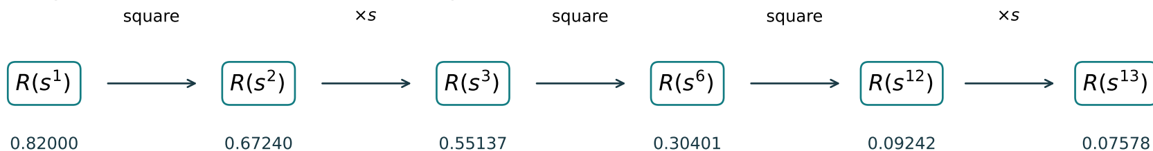
(c) Binary schedule: 13 = (1101)_2 ; five multiplications instead of twelve
