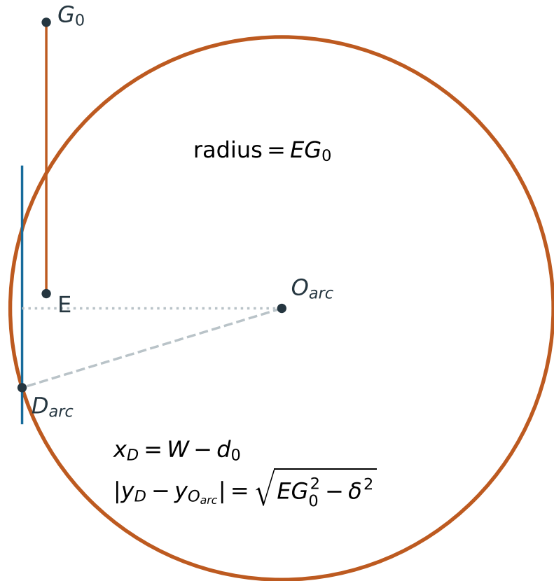
(a) A displaced center leaves a square root
