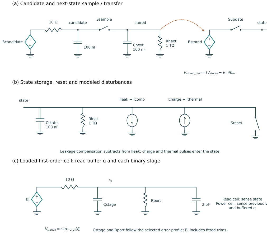
Figure 9: Electrical topology from the V30 behavioral prototype: candidate and next-state memory, explicit state disturbances and a loaded arithmetic cell. Diamonds represent behavioral voltage sources; the RC elements and switch connections are explicit in the netlist. The ADC is a separate transfer model. This realization concerns the AD map, not the fifth-order circle devices.
