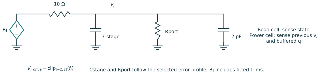
Figure 3: Electrical topology of the precision-mode SPICE model. Repeated node labels denote the same net. (a) Candidate filtering, sample storage, calibrated voltage buffer and transfer to state. (b) Explicit state capacitance, leakage resistance, net leakage/compensation current, injected disturbances and reset switch. (c) The loaded cell used for the read buffer and every centered power stage. Diamonds are behavioral voltage sources, not transistor-level amplifiers. The orange dashed arrow indicates voltage sensing, not a conductive path.
