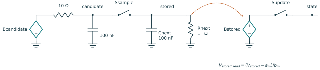
(b) State storage, reset and modeled disturbances
