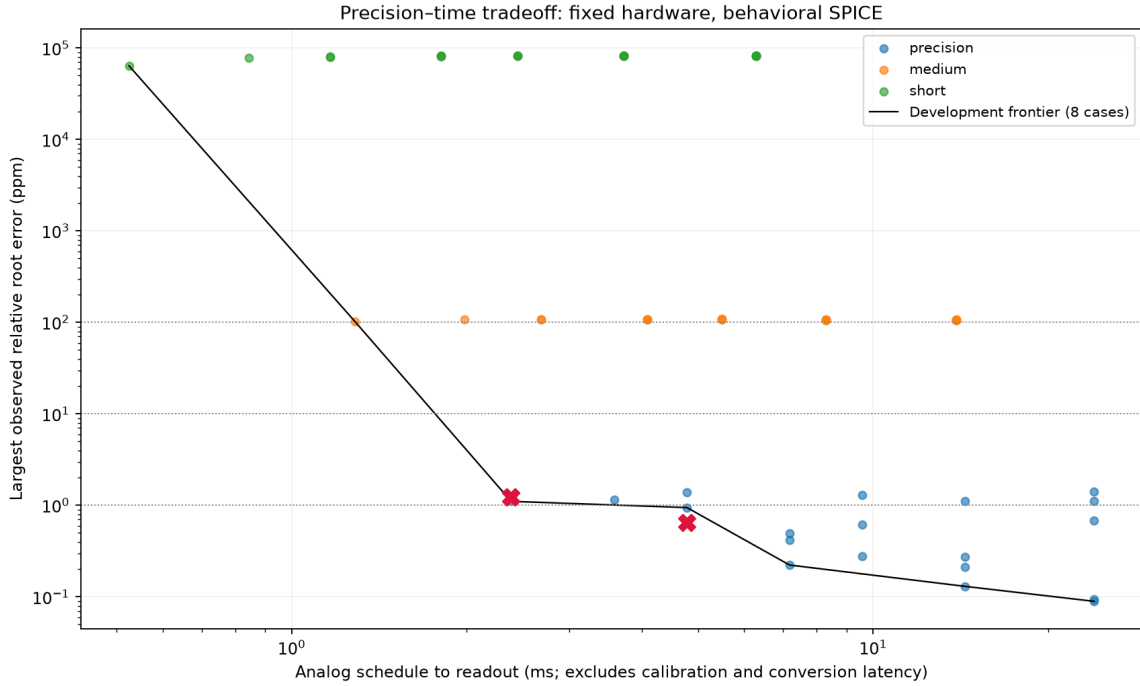
Figure 5: Largest observed error versus scheduled readout time. Colored points are fixed policies on the development set; red crosses are validation maxima. The connecting line is not an interpolated accuracy guarantee. Two more aggressive schedules have rejected trajectories and cannot enter the all-case frontier.
