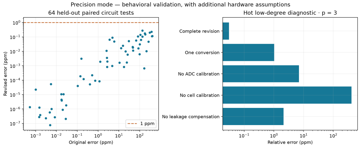
Figure 4: Left: paired precision-revision errors on 64 validation inputs. Right: one hot, low-degree diagnostic case, p = 3 , X = 0.037 , 85^\circ\text{C} . The ablation results attribute improvements within that case; they are not universal per-block error bounds.
