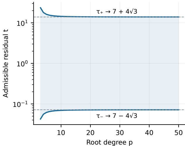
Real transverse domain \Delta > 0
