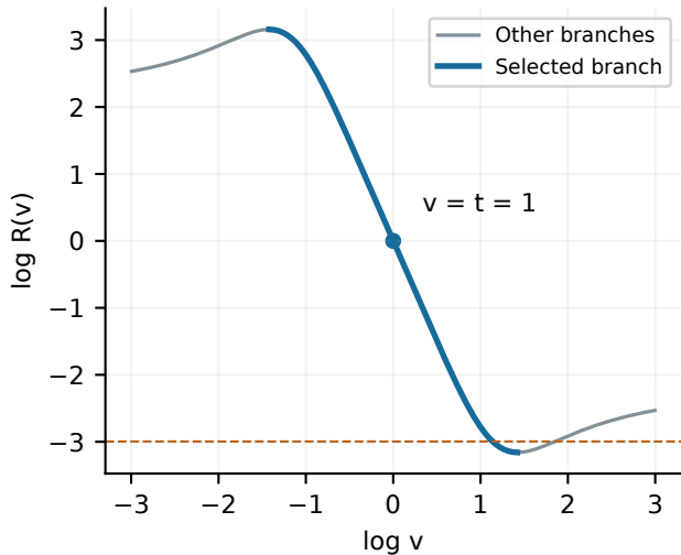
The inverse is branch-dependent ( p = 3 )
