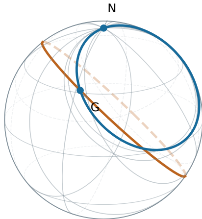
Sphere: \Gamma excludes N
