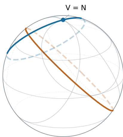
Sphere: V reaches N
