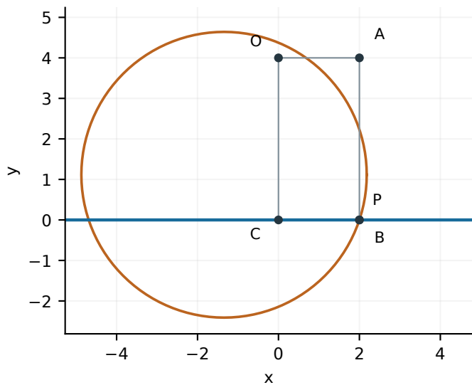
Plane: CP parallel to OA
