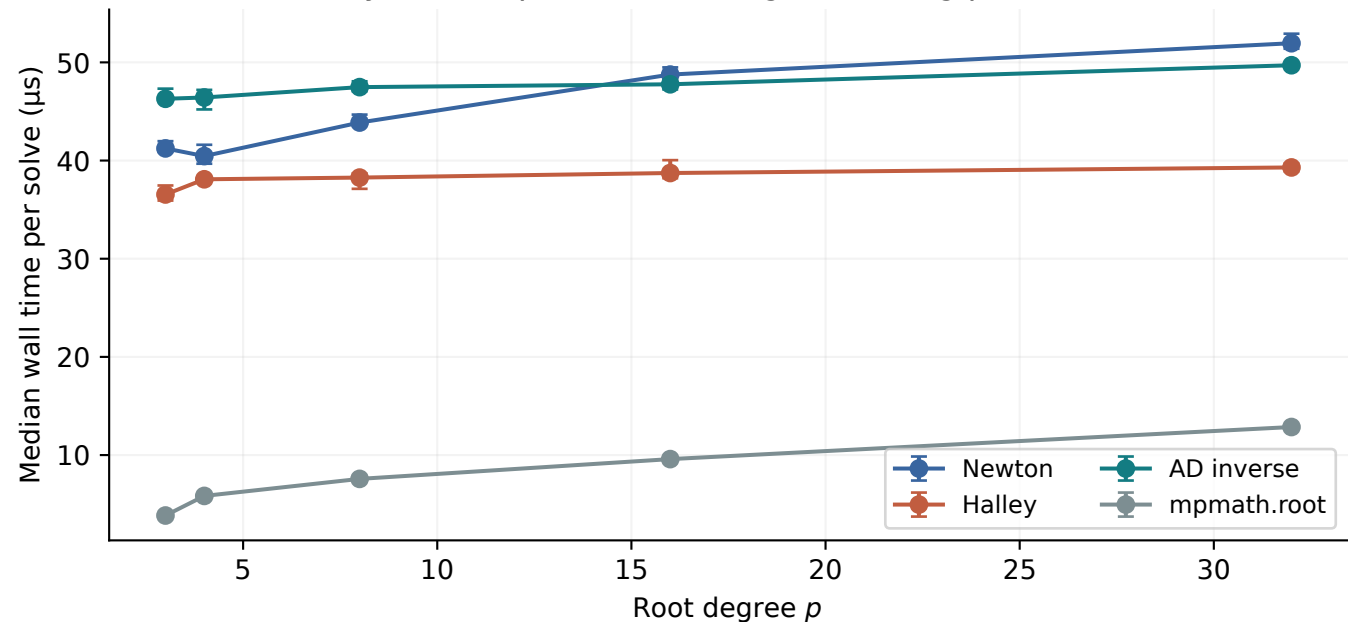
Python / mpmath • 140 digits working precision
