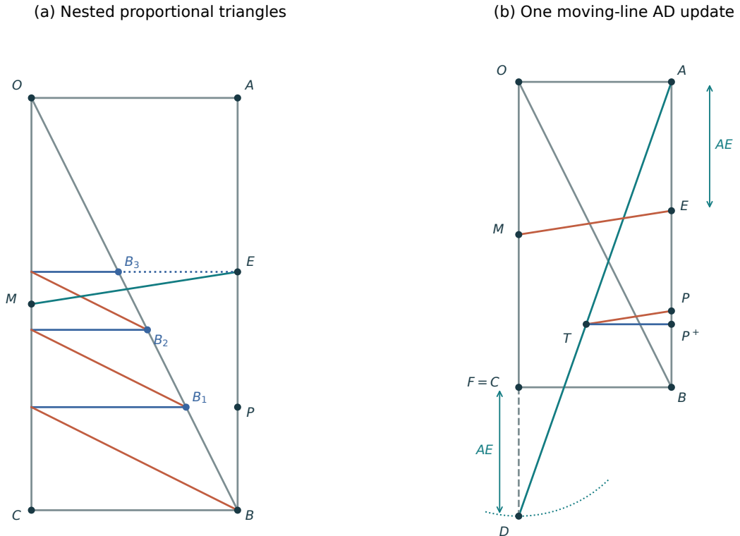
Figure 1: Geometric source of the update, retained from V17. For p = 3, X = W = 2, H = 4, s = 3/4 , the proportional chain supplies E and the moving support reports P^+ . Extended lines are allowed. The fast circuit replaces the linear-length power chain by binary arithmetic; it does not physically reproduce this drawing.
