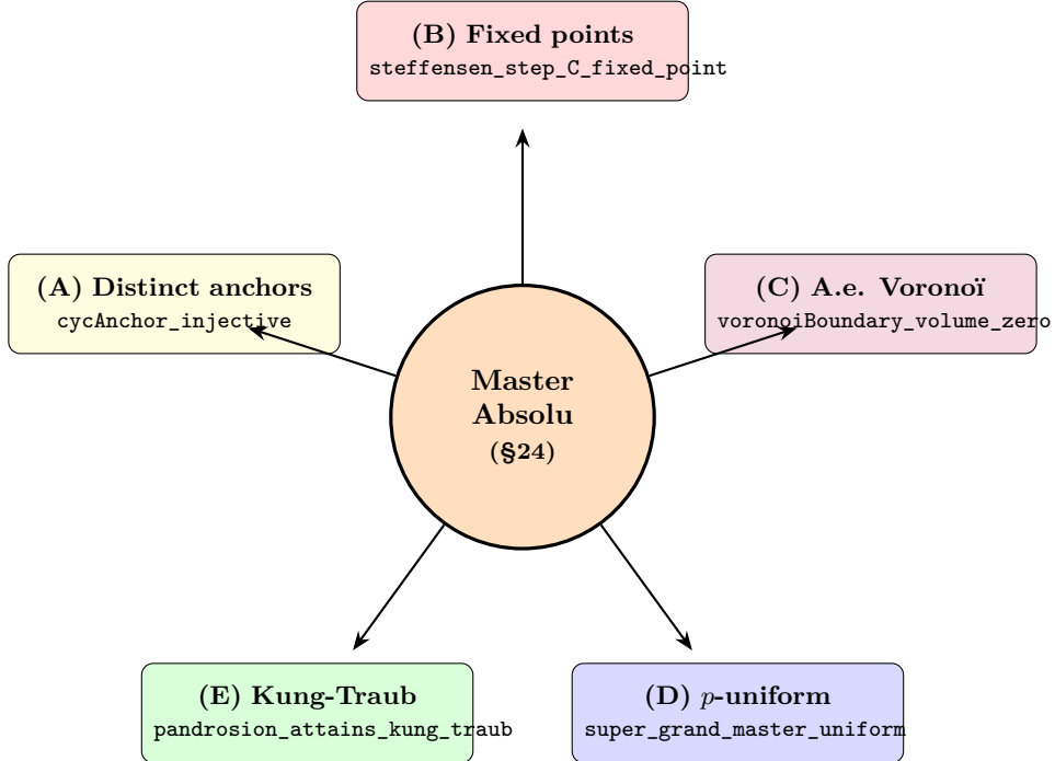
Figure 1: Master Absolu stitching. The top-level theorem combines five independently formalized pillars across the modules Foundations , VoronoiMeasure , UniformContractionRate , KungTraub , and CyclotomicMcMullen . No new lemmas are introduced in MasterAbsolu.lean .
