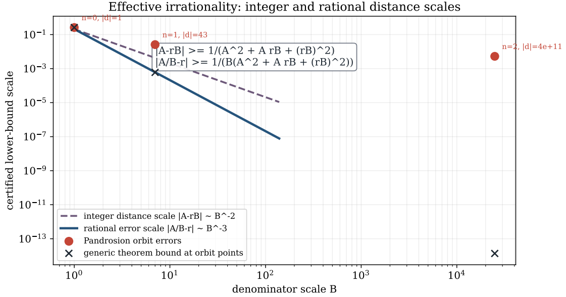
Figure 31: Effective irrationality bound. Theorem 10.1 in EffectiveIrrationality.lean turns the cubic factorisation A^3 - (rB)^3 = (A - rB)(A^2 + ArB + (rB)^2) and the discreteness of nonzero integers into an explicit lower bound for |A - rB| ; dividing by B gives the corresponding rational approximation bound for |A/B - r| . The Pandrosion norm propagation keeps this bound applicable along the integer orbit.
