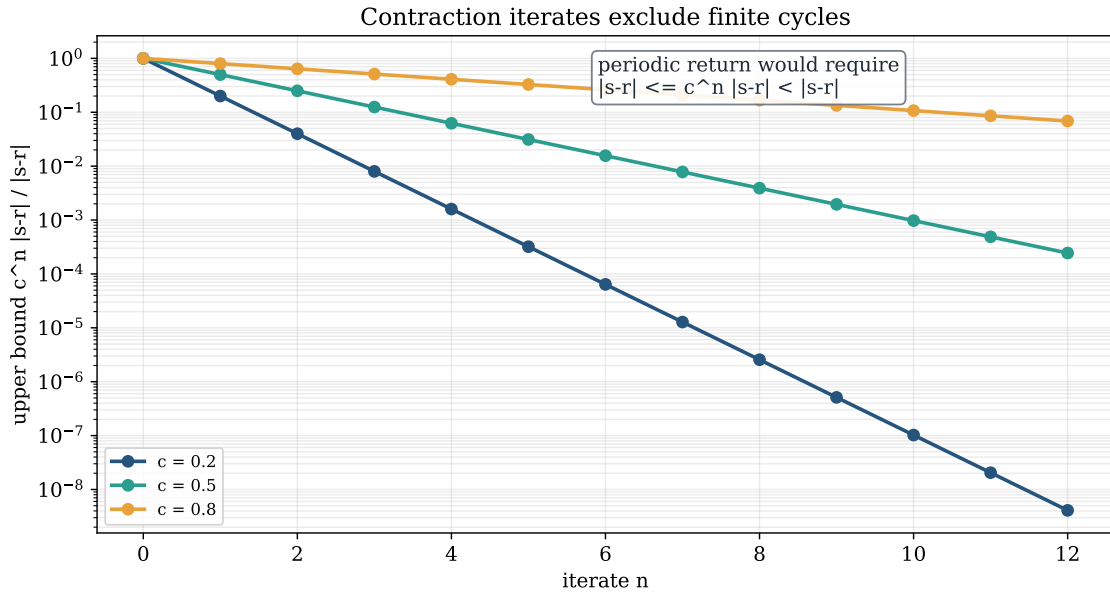
Figure 25: No periodic orbits under contraction. NoCycles.lean proves that if |f(s) - r| \leq c|s - r| with 0 \leq c < 1 , then any finite periodic return f^n(s) = s forces s = r . The figure shows why: every composed contraction multiplies the nonzero distance by c^n < 1 , contradicting exact return.
