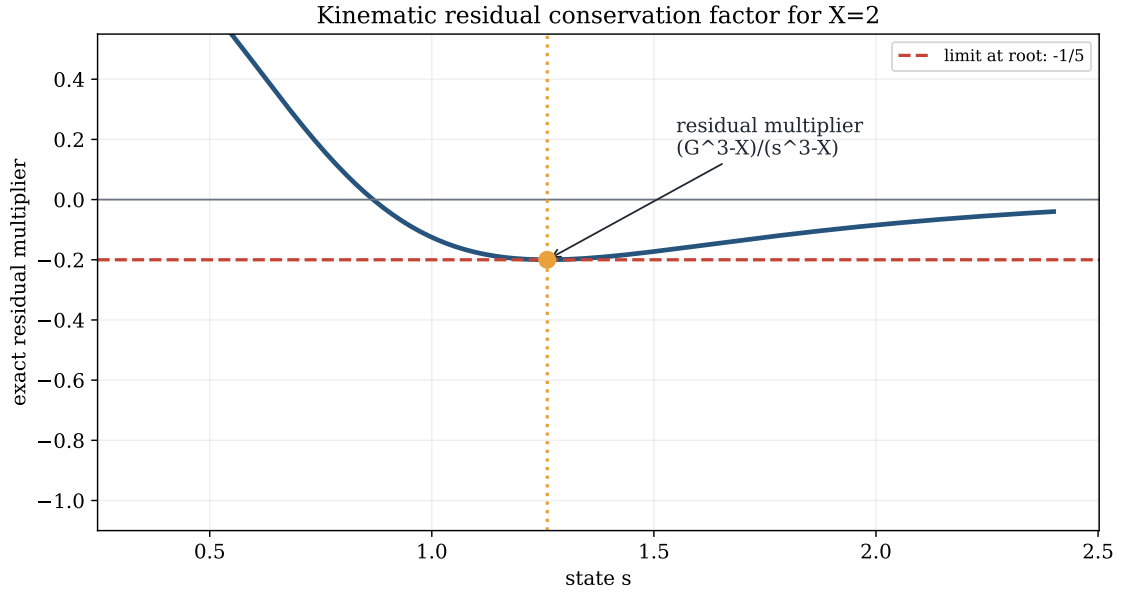
Figure 24: Kinematic residual conservation. ResidualConservation.lean certifies the exact factorisation G^3 - X = (s^3 - X)\Phi(s, X)/(3s^3 + 2X)^3 . The plotted multiplier for X = 2 crosses the fixed point with limiting value -1/5 , matching the derivative theorem and giving the residual-level explanation of the convergence mechanism.
