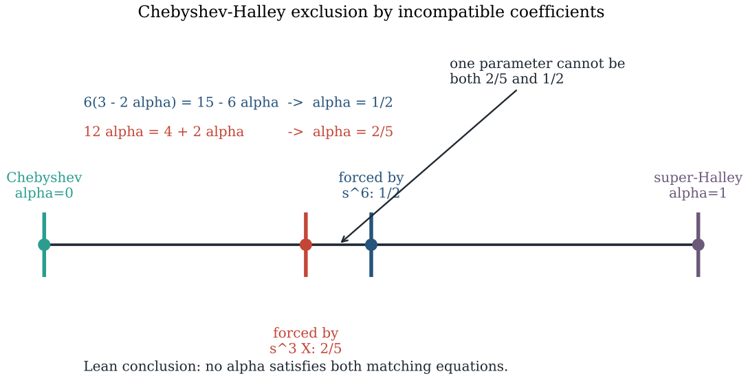
Figure 23: Chebyshev–Halley exclusion. ChebyshevHalleyExclusion.lean proves that matching Pandrosion to the one-parameter Chebyshev–Halley family would force two incompatible values of the same parameter: \alpha = 1/2 from the s^6 coefficient and \alpha = 2/5 from the s^3X coefficient. Hence Pandrosion is not any member of that classical family.
