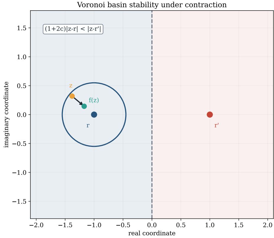
Figure 28: Voronoi basin stability. Theorem 5.5 links algebraic contraction to geometric basin persistence: if z is deep enough in the Voronoi cell of r , then the contracted point f(z) remains closer to r than to a competing anchor r' . This is the geometric bridge between the contraction proof and the multi-start basin architecture.
