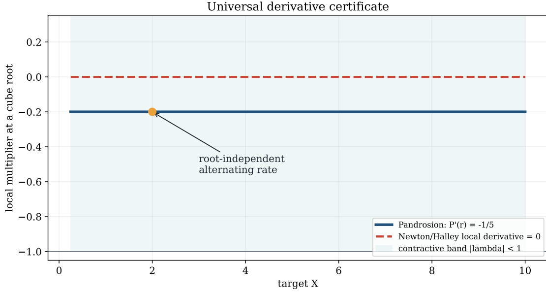
Figure 22: Universal derivative certificate. Theorem 2.4 and HalleyComparison.lean prove that the local multiplier of the cubic Pandrosion map at every nonzero cube root is exactly -1/5 , independently of the target X . The negative sign explains the alternating approach pattern; the absolute value gives a certified contraction rate.
