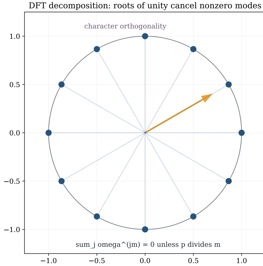
Figure 30: DFT character orthogonality. DFTDecomposition.lean proves the roots-of-unity cancellation law: \sum_{j=0}^{p-1} \omega^{jm} is p when p \mid m and 0 otherwise. This supplies the spectral bookkeeping used by the Fourier and descent modules.
