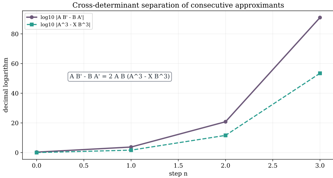
Figure 27: Cross-determinant separation. Theorem 6.2 proves AB' - BA' = 2AB(A^3 - XB^3) . This locks the separation of consecutive rational approximants to the same cubic norm that drives the Thue-style amplification, so distinctness is carried by an explicit polynomial certificate.
