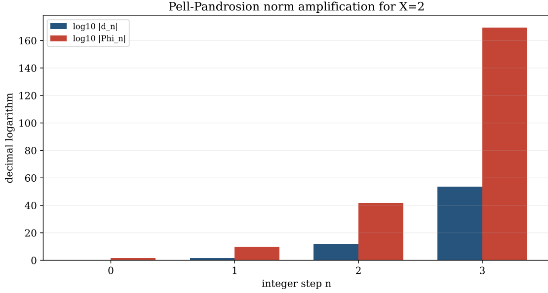
Figure 26: Pell–Pandrosion integer amplification. Theorem 4.1 and ThueBridge.lean prove the exact law d_{n+1} = d_n \Phi_n for d_n = A_n^3 - X B_n^3 . For X = 2 , the logarithmic growth of both the norm and the amplification factor becomes enormous after only a few certified integer steps.
