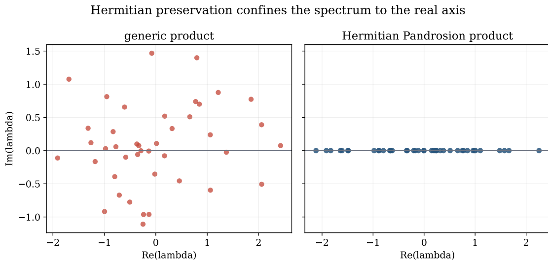
Figure 29: Hermitian preservation. Theorem 7.2 and HermitianPreservation.lean prove that the Pandrosion numerator and denominator product preserves the Hermitian condition when the inputs are Hermitian and commute. The visual consequence is spectral confinement to the real axis, unlike a generic complex product.
