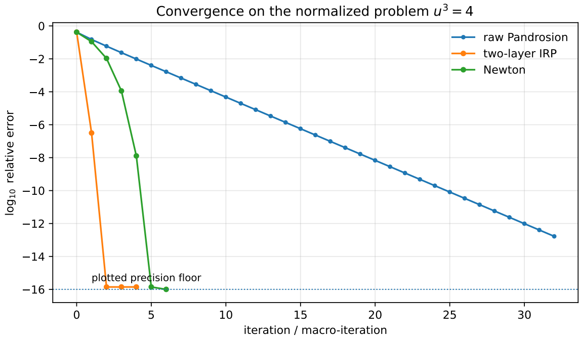
Figure 5: Iteration histories on the normalized problem u^3 = 4 . Raw Pandrosion is linear, Newton is quadratic, and two-layer IRP reaches the plotted precision floor in a few renormalized macro-updates.
