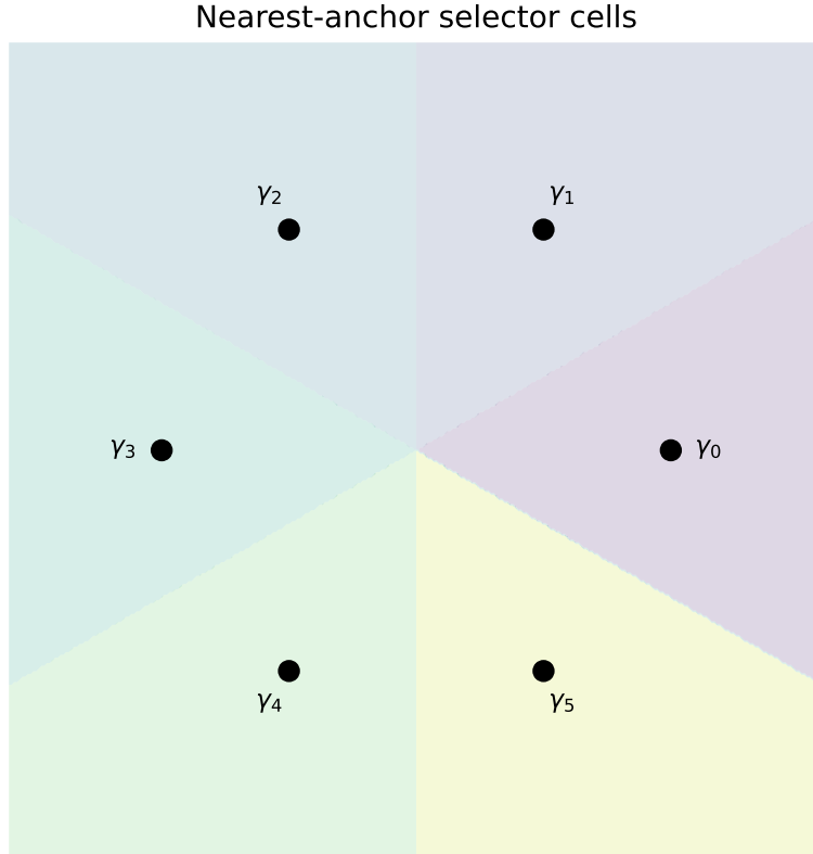
Figure 7: The nearest-anchor selector partitions the complex plane into Voronoi cells. The selector is simple and locally stable away from the cell boundaries.
