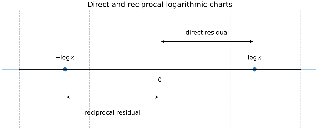
Figure 3: Direct and reciprocal logarithmic charts. The affine chart uses \log y_+(B) = \log x - p \log B , while the reciprocal chart uses \log y_\infty(B) = -\log x - p \log B . Chart selection chooses the line whose normalized logarithmic target lies closest to 0.
