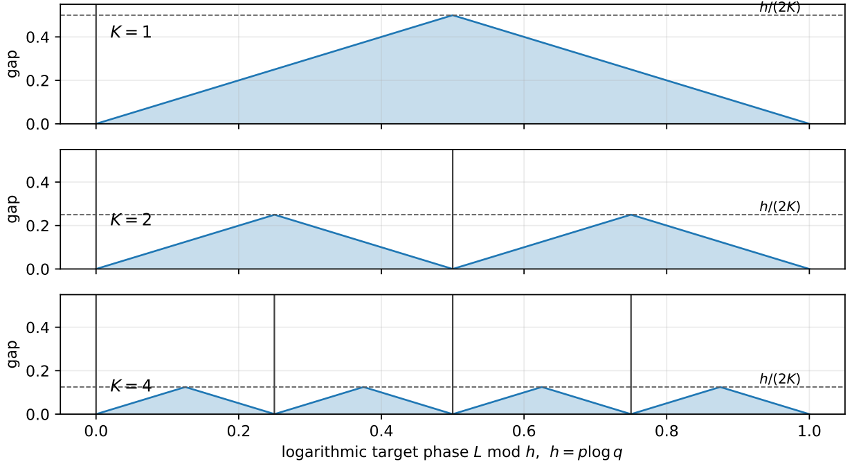
Figure 4: The scale-lattice theorem in one picture. For a logarithmic period h = p \log q , equally spaced K -phase palettes have covering radius h/(2K) , and no K -point palette can do better.
