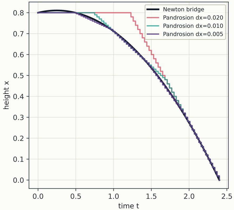
Weak-field Pandrosion shadow recovers Newton's parabolaNewtonian limit benchmark
