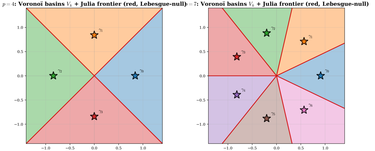
Figure 5: Voronoi decomposition of \mathbb{C} for cyclotomic anchors at p = 4 and p = 7 , x = 2 . Each colored region V_k is the basin of attraction of \gamma_k under the selector. The red frontier is the Voronoi boundary of the cyclotomic anchor set; it is Lebesgue-null.
