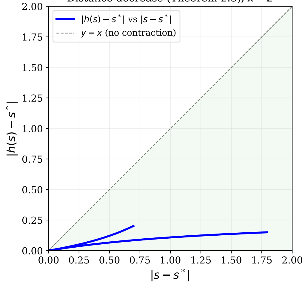
Distance decrease (Theorem 2.5), x = 2
