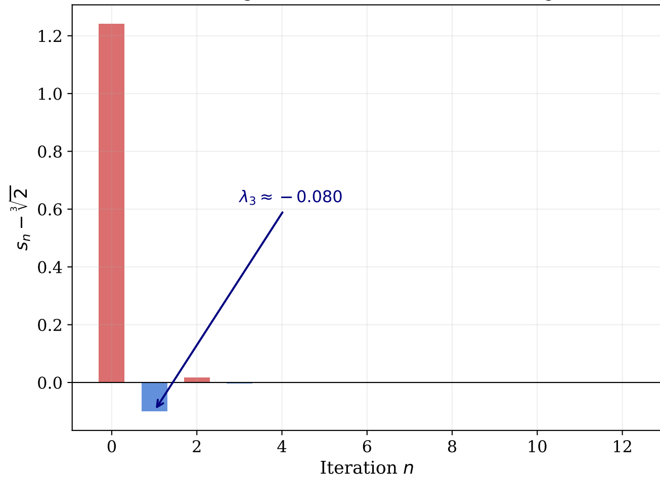
Oscillation signature (Theorem 2.7): alternating error
