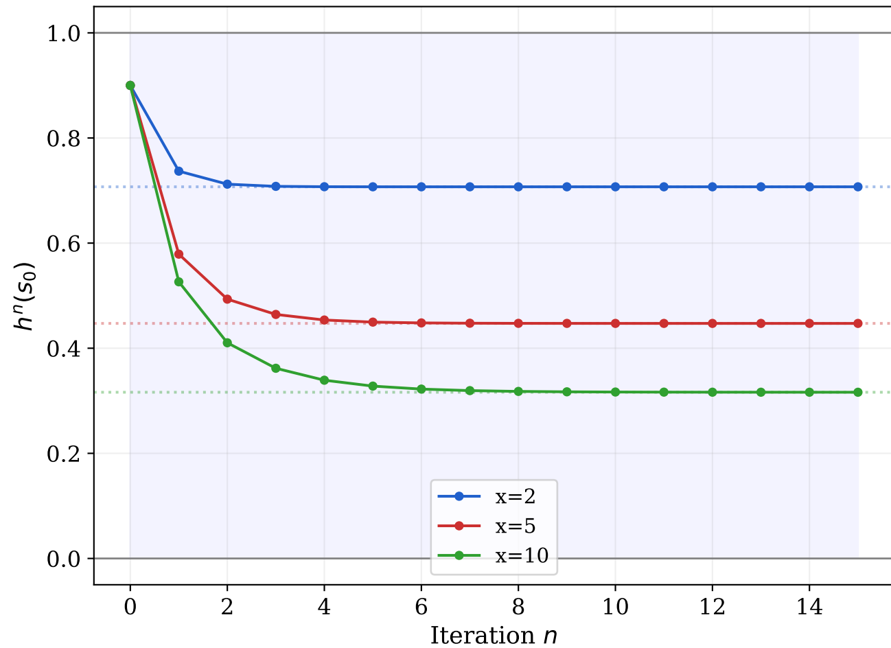
Orbit invariance (Theorem 2.6): h^n(s_0) \in (0, 1)
