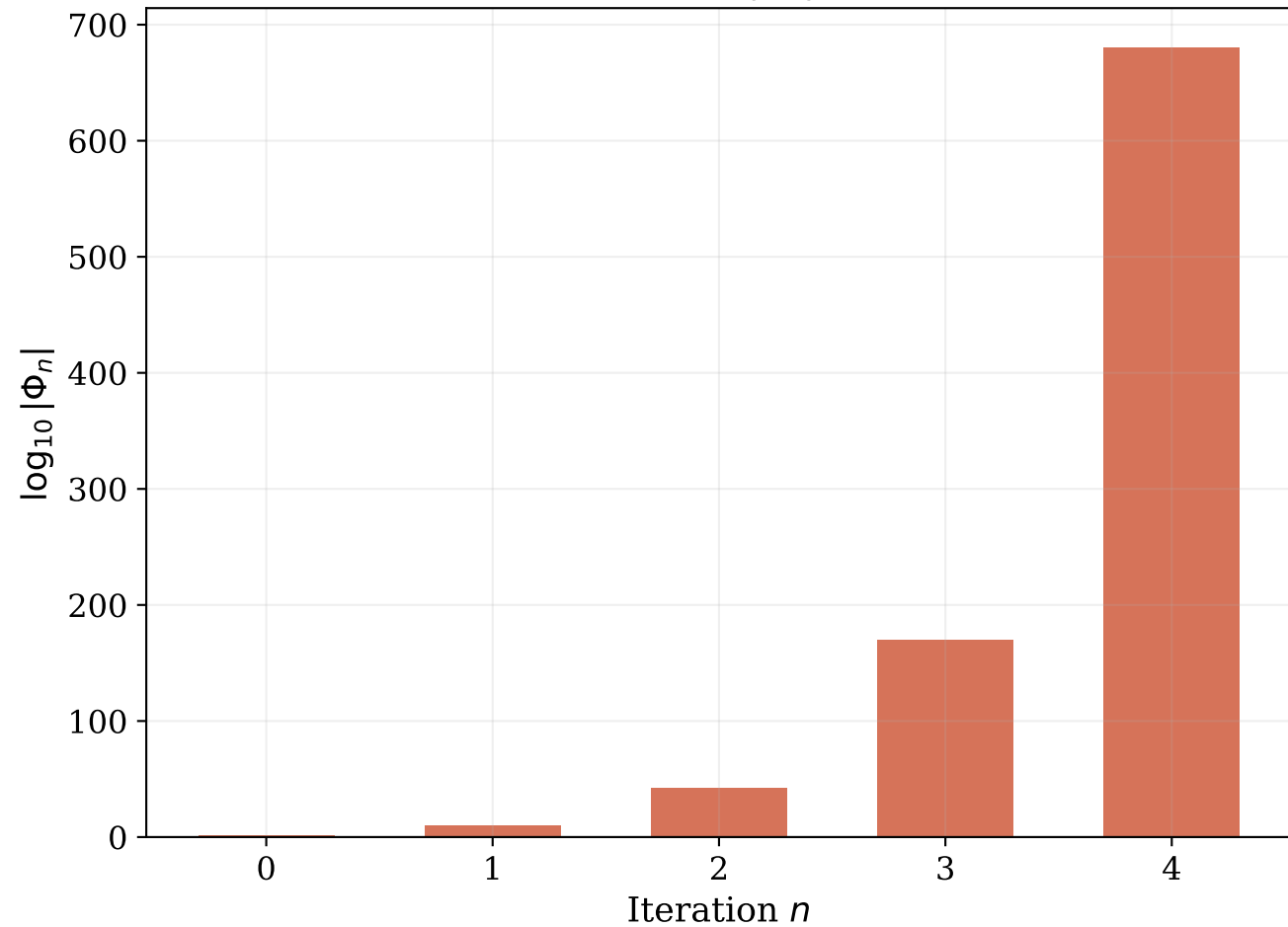
Polynomial factor |\Phi_n| (degree 9)
