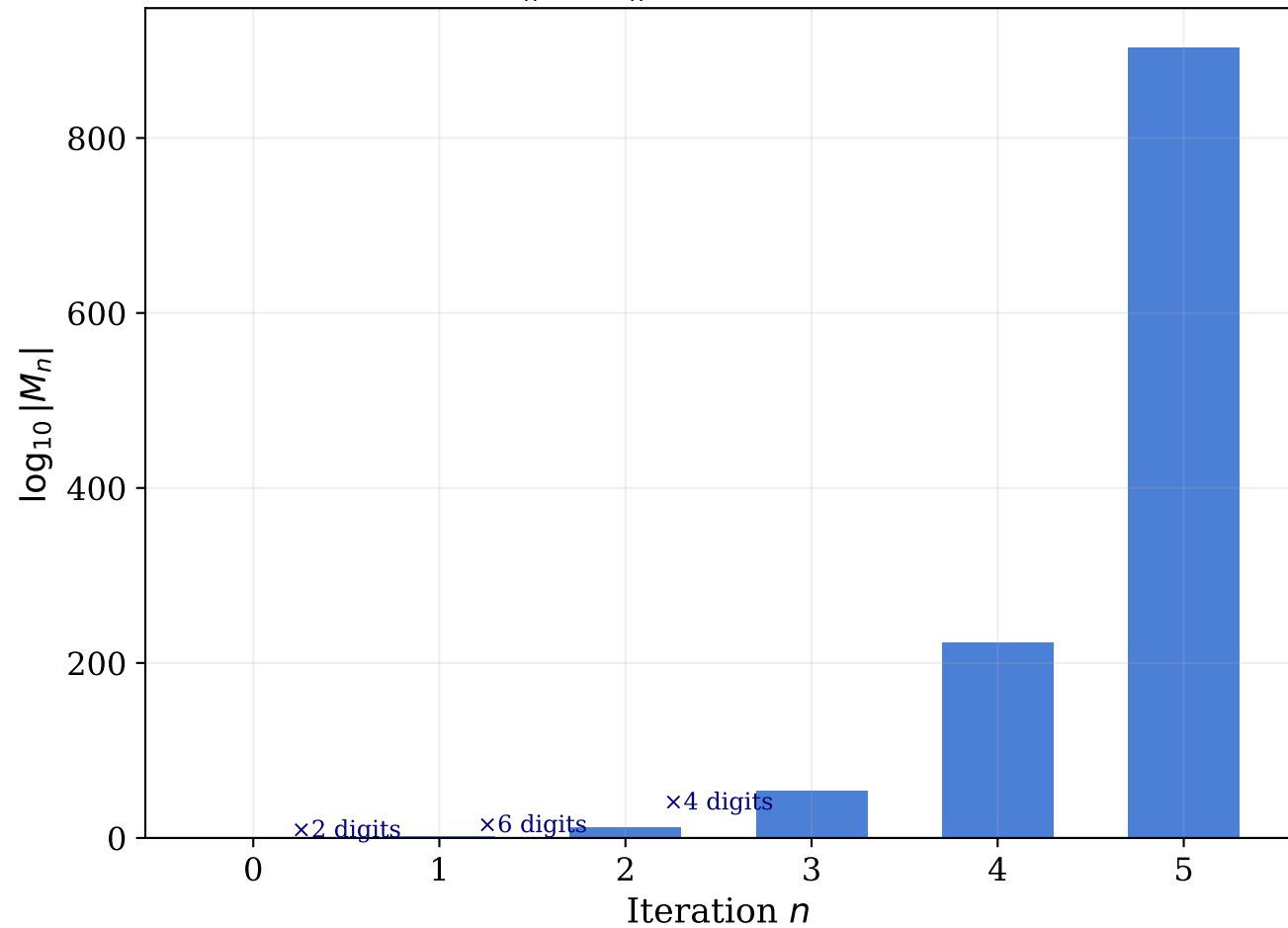
|M_n| = |A_n^3 - 2B_n^3| : multiplicative growth
