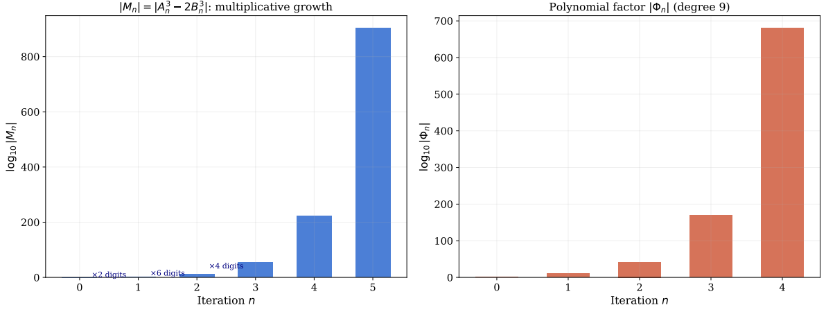
Figure 6: Left: Growth of |M_n| = |A_n^3 - 2B_n^3| on a logarithmic scale. Each iteration approximately cubes the number of digits, consistent with the degree-9 polynomial factor in Theorem 3.1. Right: The polynomial factor |\Phi_n| at each step, showing that the multiplicative amplification grows explosively while keeping the factorisation exact.
