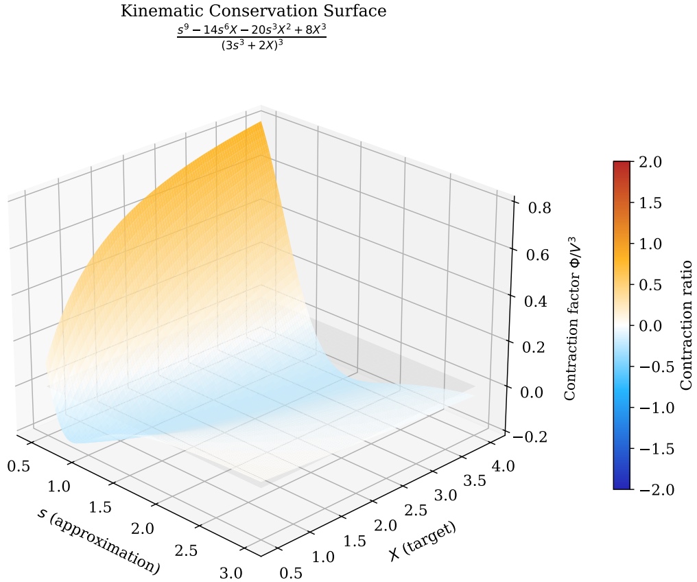
Figure 3: 3D Kinematic Conservation Surface . The contraction ratio \Phi(s, X)/(3s^3 + 2X)^3 governs the error decay at each step. The surface crosses zero along the curve s^3 = X (the exact roots), confirming that the iteration converges from both directions. The steep gradients near the root manifold explain the cubic convergence speed.
