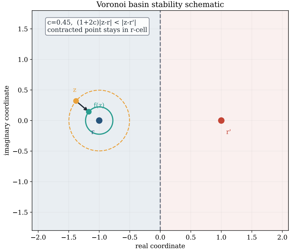
Figure 28: Voronoi basin stability. This schematic combines the 2D convexity of Voronoi half-planes from VoronoiInvariance.lean with the distance inequality of Theorem 5.5: if z is deep enough in the cell of r , then a contraction toward r leaves the next point closer to r than to a competing anchor r' . The formal basin-stability theorem is stated as a real distance inequality; the displayed plane is the geometric interpretation used by the multi-start architecture.
