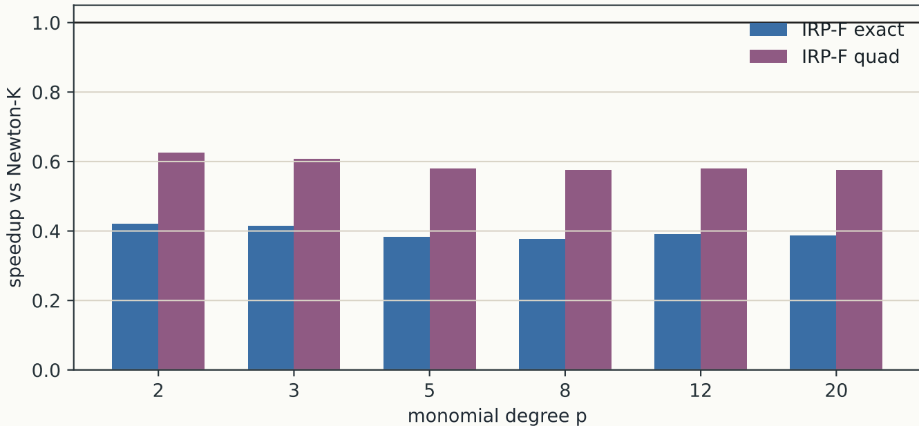
Fused IRP wall-clock ratio on calibrated scalar roots
