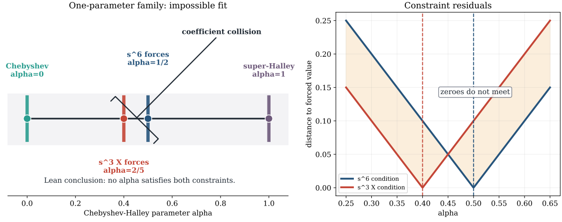
Figure 23: Chebyshev–Halley exclusion. ChebyshevHalleyExclusion.lean proves that matching Pandrosion to the one-parameter Chebyshev–Halley family would force two incompatible values of the same parameter: \alpha = 1/2 from the s^6 coefficient and \alpha = 2/5 from the s^3X coefficient. Hence Pandrosion is not any member of that classical family.
