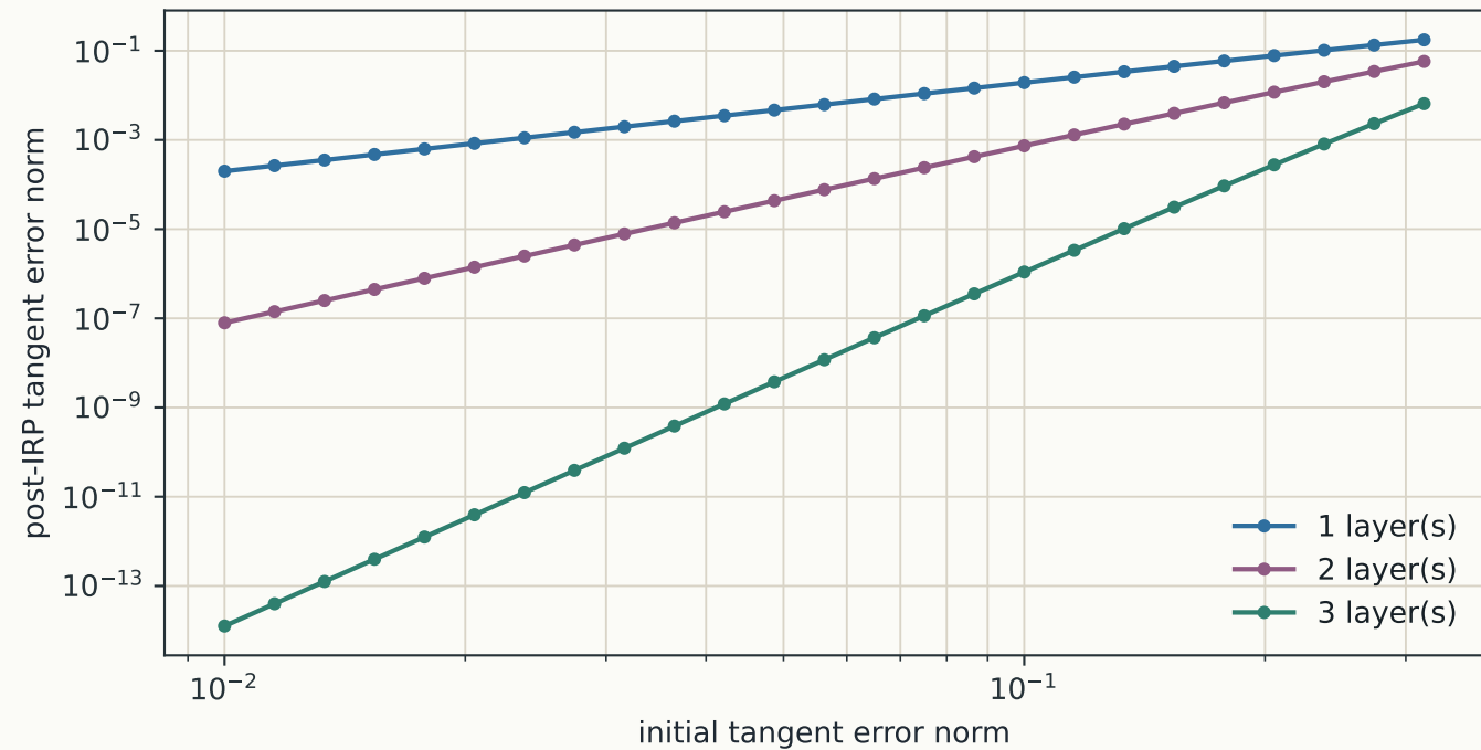
Poincare-ball realization of Hadamard IRP local order
