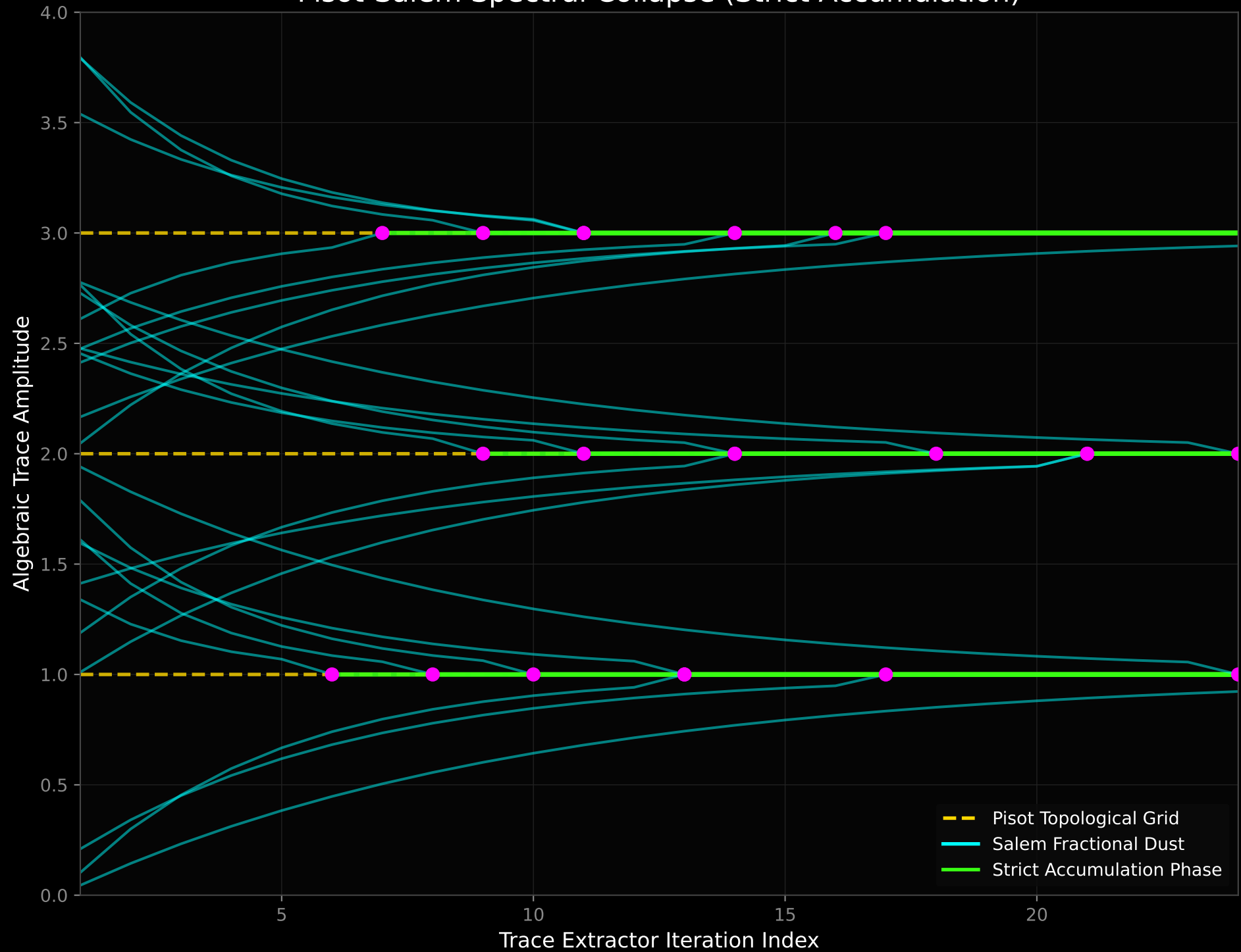
Pisot-Salem Spectral Collapse (Strict Accumulation)
