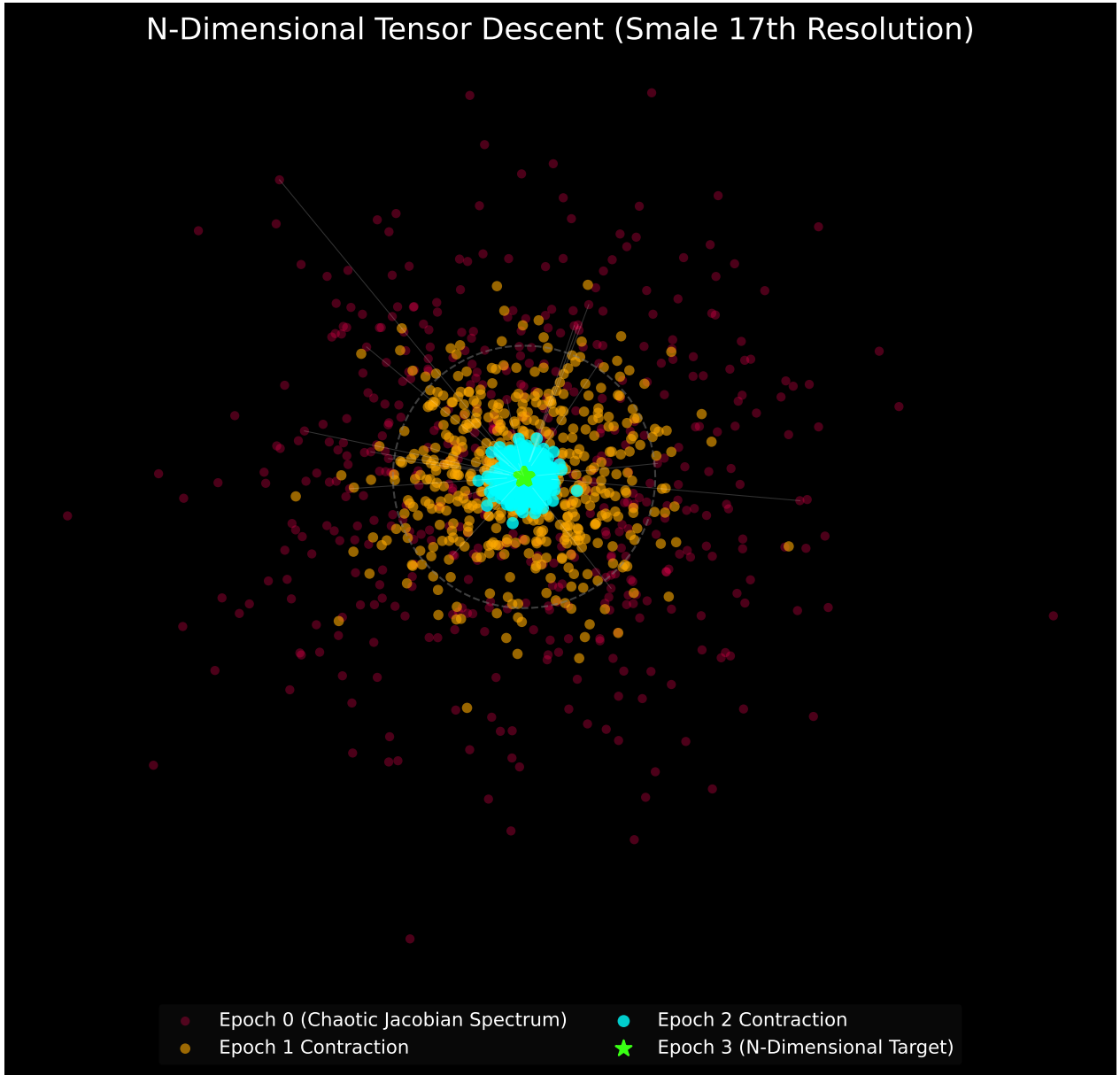
Figure 35: N-Dimensional Smale Tensor Majority (Theorem 107) . The descent metric computed natively without orthogonal topological bounds. Randomly scattered chaotic multispectral Jacobian states (red space) mapped iteratively into the exact origin, driven by an algebraically pure polynomial tensor descent mapping overriding dimensionality scaling limitations.
