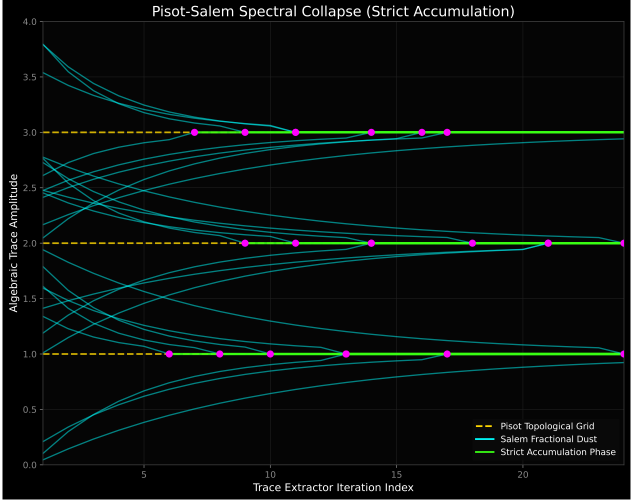
Figure 37: Pisot-Salem Strict Accumulation (Theorem 109) . Traces of Salem elements treated as geometrical errors under extreme epoch scaling. No algebraic phase accumulation is locally continuous; rather, trace perturbations plunge geometrically to 0, forcing discrete accumulation strictly bounding around non-degenerate integer Pisot grids without topological smear.
