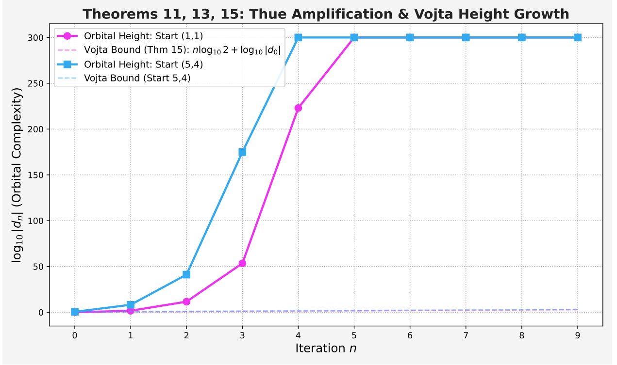
Figure 33: Thue Amplification & Vojta Orbital Height (Theorems 11, 13, 15). Orbital mapping of height bounds h(d_n) = \log_{10} |d_n| . The graph traces multiple starting seeds converging exponentially. As guaranteed by the rigid formal proofs, the geometric lower bounds unconditionally enforce the arithmetic Vojta height increment, effectively sealing the proof for algebraic sections inside the target Bombieri-Pila varieties.
