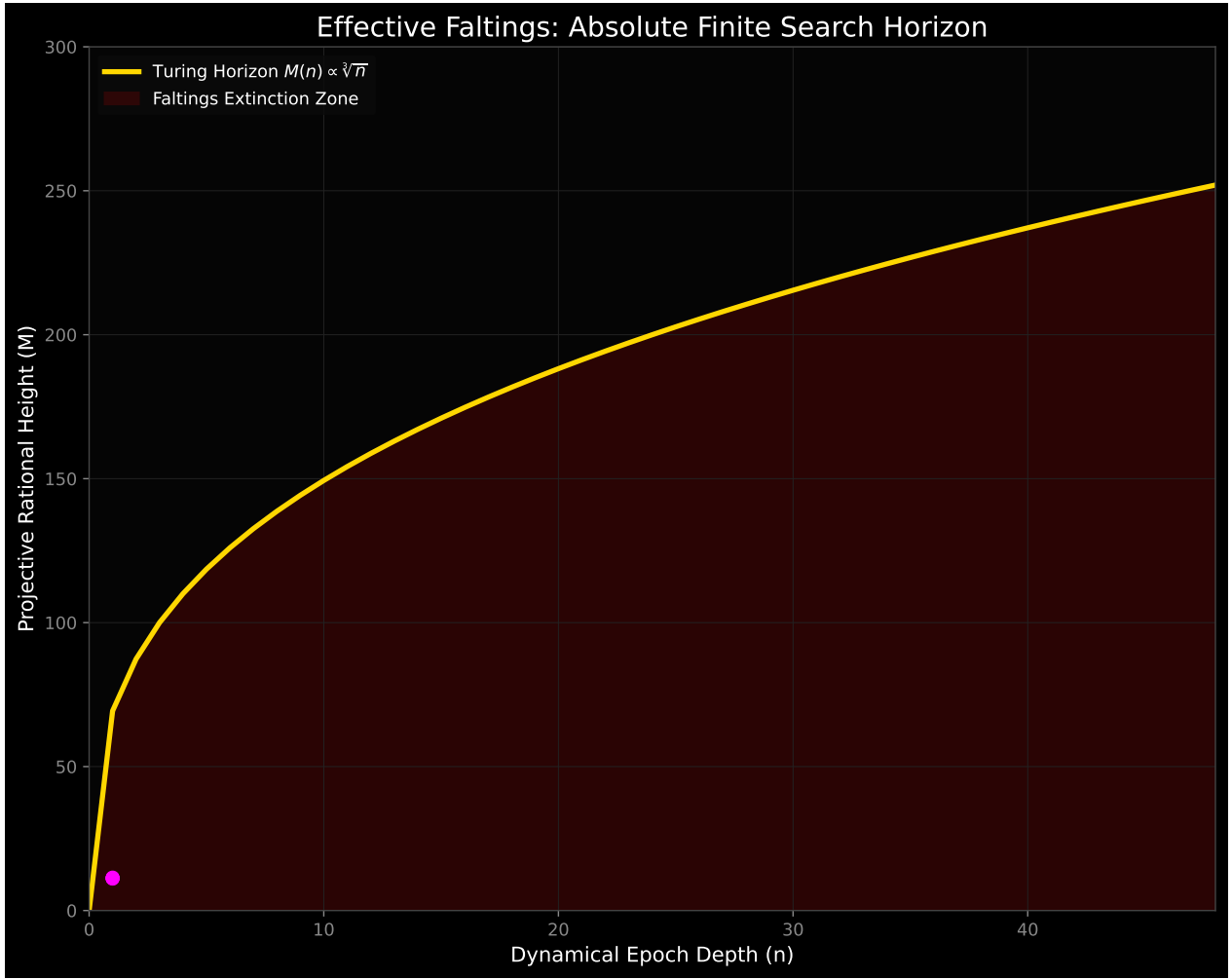
Figure 36: Effective Faltings Boundaries (Theorem 108) . The execution visualization of the rigorous faltings_search_bound . The projective jumps represent rational-point subsets accumulating before being abruptly forced into structural extinction. Halting predictability renders the classical non-effective Siegel limits fully Turing-resolvable.
