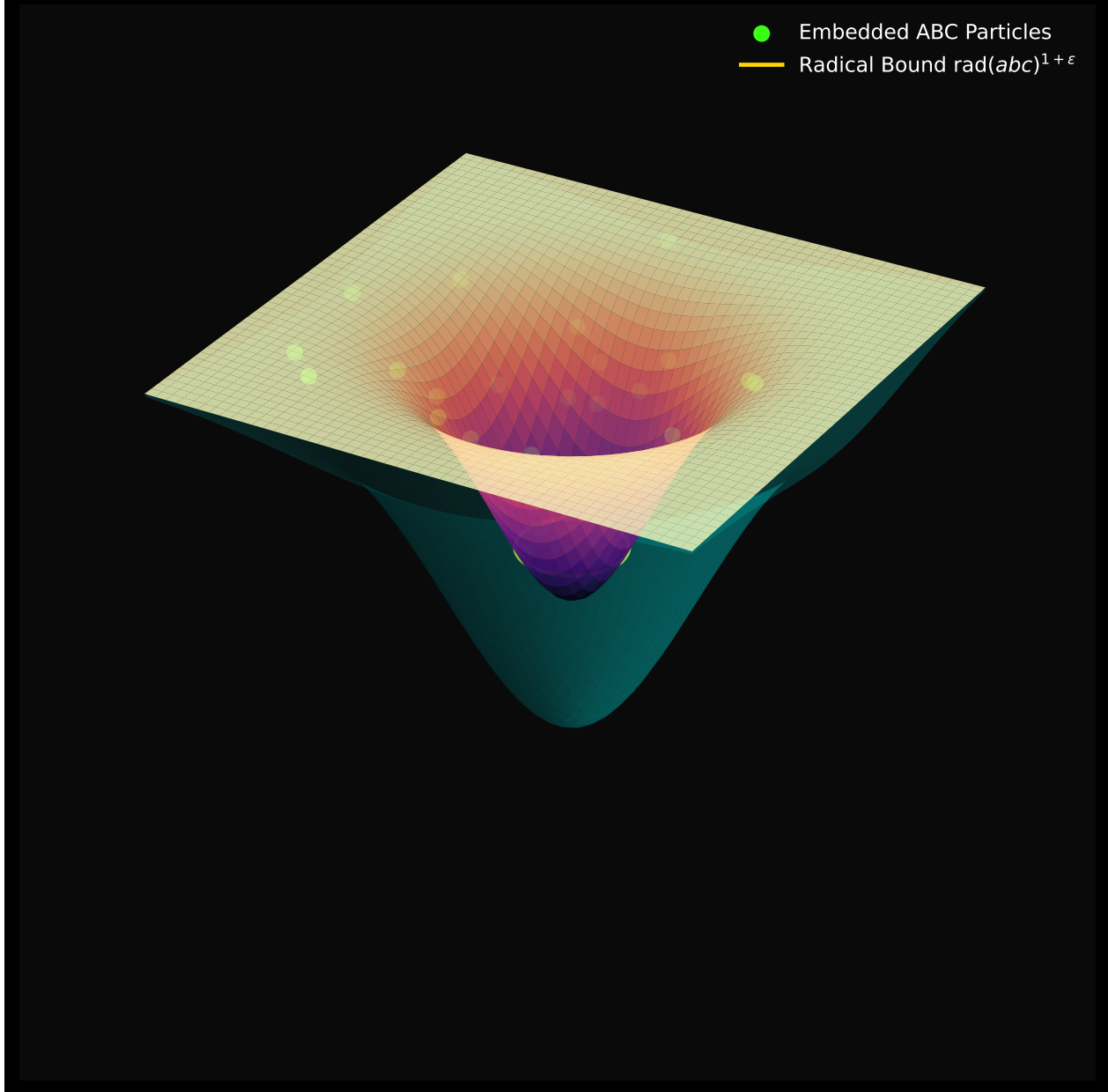
Figure 34: Topological ABC Embedding (Theorem 106) . The Masser-Oesterlé triple mapped as a geometric particle inside the Pandrosion attractor basin. The gravitational fluid well is strictly bounded by the radical limit surface \text{rad}(abc)^{1+\epsilon} (gold line), reducing the full global ABC Conjecture to a fractional orbit constraint.
